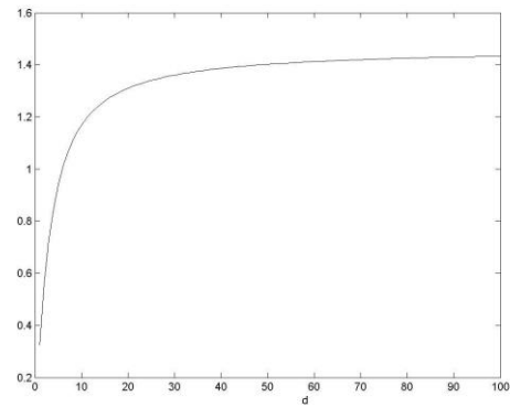
Fig.2 \min \lambda(-A+D) versus the control gains
