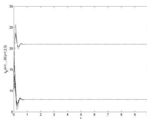
Fig.8 Convergence of pinning 5 “smallest” nodes
