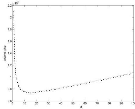
Fig.6 Control cost of pinning the “smallest” nodes
