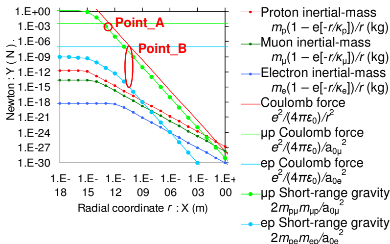
FIG. 3. The scalable inertial mass of fermions, and the Coulomb force and the short-range gravity of a combination thereof. The red / green / blue dotted lines are the scalable inertial mass curves of each fermion. The solid lines are the line that Coulomb force. The Yellow-green / light-blue dotted lines (proton-muon, proton-electron) are the short-range gravity line.
