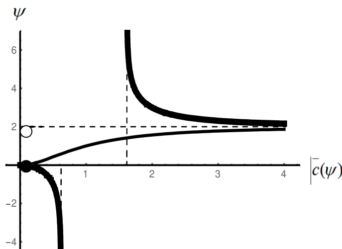
Figure.3.2. The graph of the dependence of the parameter of self-organization \psi from the module |\bar{c}(\psi)| of the normalized Fibonacci light velocity in vacuum \bar{c}(\psi) .
