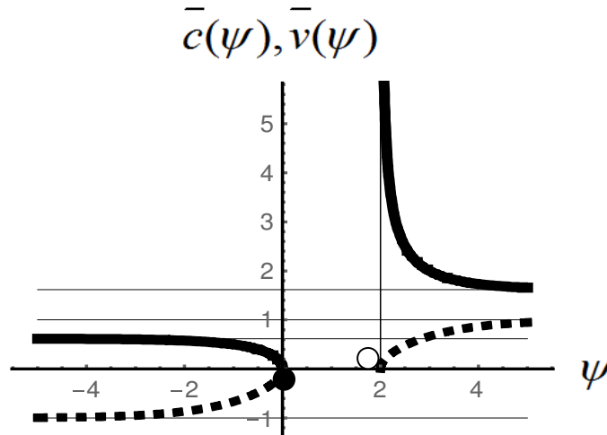
Figure 2.2 . The graph \bar{c}(\psi) (the black curves ) and the graph \bar{v}(\psi) (the dashed curves ), where the parameter \psi is in limits \{-\infty < \psi < 0\} \cup \{2 < \psi < +\infty\} . The symbols \bullet and \circ correspond to the bifurcation points \psi = 0 and \psi = 2 .
