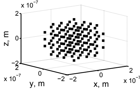
Figure 1: The schematic representation of the spherical cluster made of 123 small cubes. The period of the cluster is d=2.2L , and the characteristic size of the cubes is L = 25 nm.
