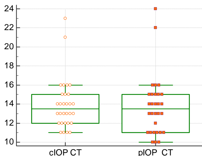
Figure 2 Intraclass correlation coefficient of central and peripheral IOP in diabetics
