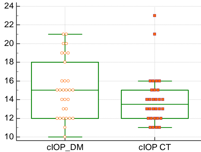
Figure 7 Showing intraclass correlation coefficient of central IOP in DM and CT
