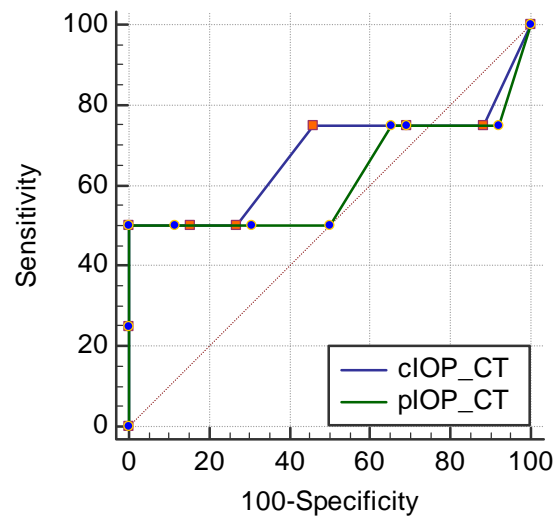
Figure 5 Comparison of ROC curves of central and peripheral IOP in controls
