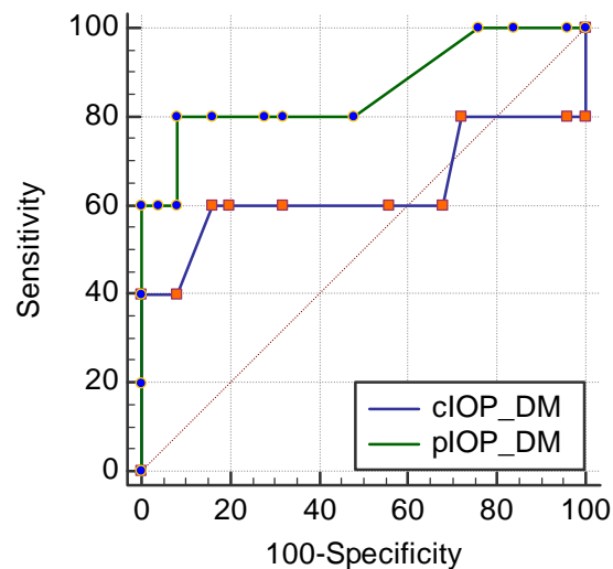
Figure 4 Comparison of ROC curves of central and peripheral IOP in diabetics
