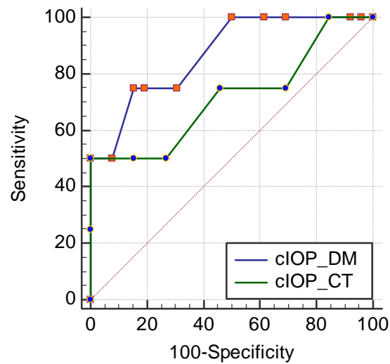
Figure 9 Comparison of ROC curves of central IOP in diabetics and controls
