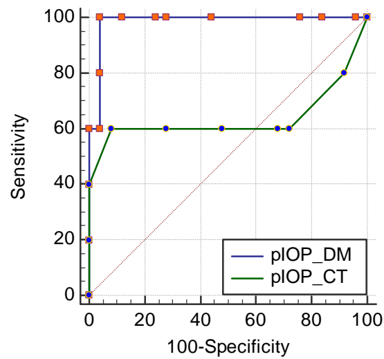
Figure 10 Comparison of ROC curves of peripheral IOP in diabetics and controls
