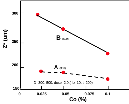
Fig.10 Same as Fig. 9 but for Z^* versus C_0 for UV light intensity of I_0=10 \text{mW}/\text{cm}^2 , and exposure time t=200\text{s} (or dose of 2.0 \text{J}/\text{cm}^2 ).
