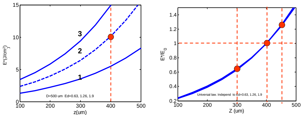
Fig. 2. The safety dose ( E^* , left figure) and normalized safety dose ( E^*/E_0 , in right figure) versus z for C_0 = 0.1\% , D = 500 \mu\text{m} , quantum yield \phi = 0.1 and E' = (0.63, 1.26, 1.9) \text{ J/cm}^2 , for curves (1,2,3) in left figure, where the red dot (in left figure) represents E^* = E_0 at the reference point ( z = 400 \mu\text{m} and E' = 1.26 \text{ J/cm}^2 ).
