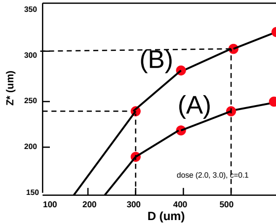
Fig. 11 Cross linking depth ( Z^* ) versus diffusion depth ( D ) for dose of 2.0 \text{J}/\text{cm}^2 , curve (A) and 3.0 \text{J}/\text{cm}^2 , curve (B), C_0=0.1\% and quantum yield \phi=0.1
