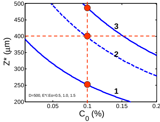
Fig. 6. Same as Fig. 5, but for D=500 \mu\text{m} and E^*/E_0=(0.5, 1.0, 1.5) for curve (1,2,3).
