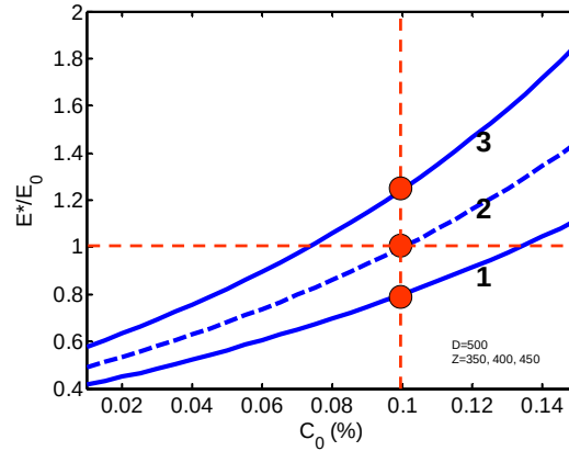
Fig. 3 The normalized safety dose ( E^*/E_0 ) versus C_0 for D=500 \mu\text{m} and z = (350, 400, 450) \mu\text{m} , for curve (1,2,3).
