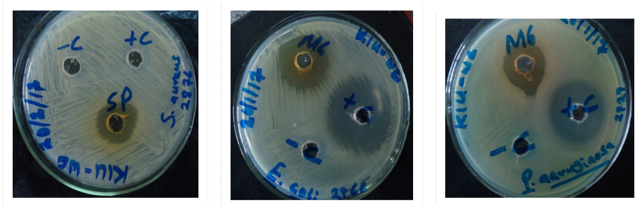
Fig. 2: Secondary screening. Antibacterial activity of ethanol extracts of BRWDSc (SP) and KBMWDSb6 (M6) using well diffusion method against resistant bacteria with both positive and negative controls
