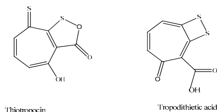
Fig. 3. The chemical structure of TDA
