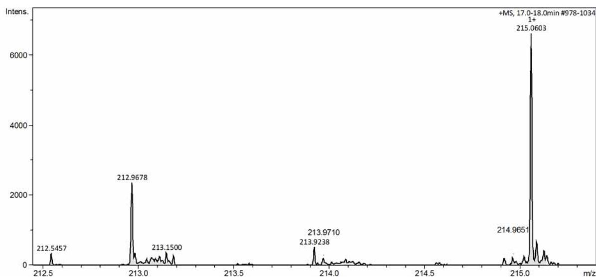
Fig. 6. LC-MS analysis of TDA produced by the strain Pseudovibrio sp. rh17: chromatographic profile (at the top) and corresponding MS spectra in positive ion mode (at the bottom).
