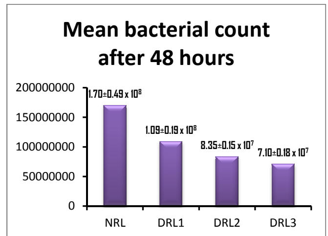
Fig. 4: Total Heterotrophic Bacterial Count after 48 hours of incubation
