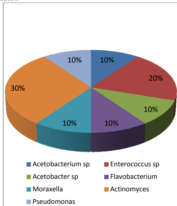
Fig. 6: Percentage Occurrence of bacterial isolates in the rubber samples
