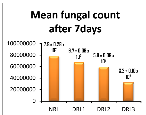
Fig. 5: Total Heterotrophic Fungal Count after 7 Days of Incubation
