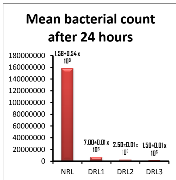
Fig. 3: Total Heterotrophic Bacterial Count after 24 hours of incubation
