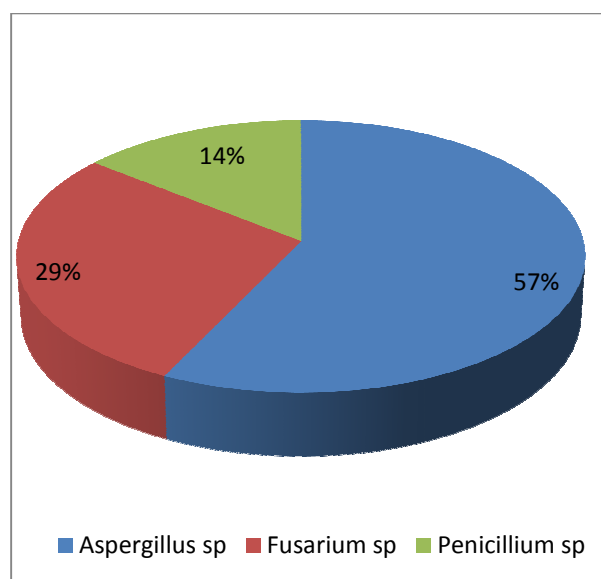
Fig. 7: Percentage occurrence of mould isolates in rubber samples
