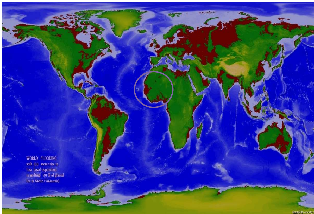
Figure 2. Affected Regions at Sea Level Rise (100 meters) 1
