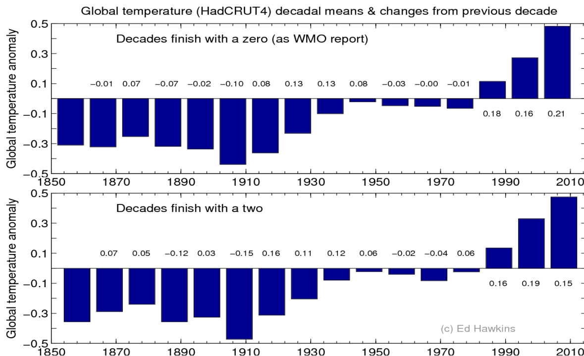
Figure 3. Global Temperature From 1850-2010 2
