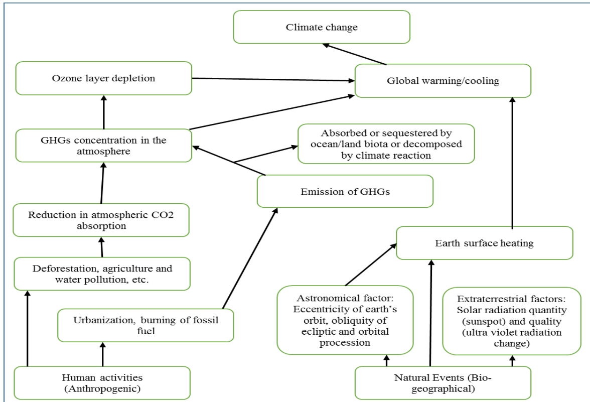
Figure 1. Causal Factors of Climate Change
