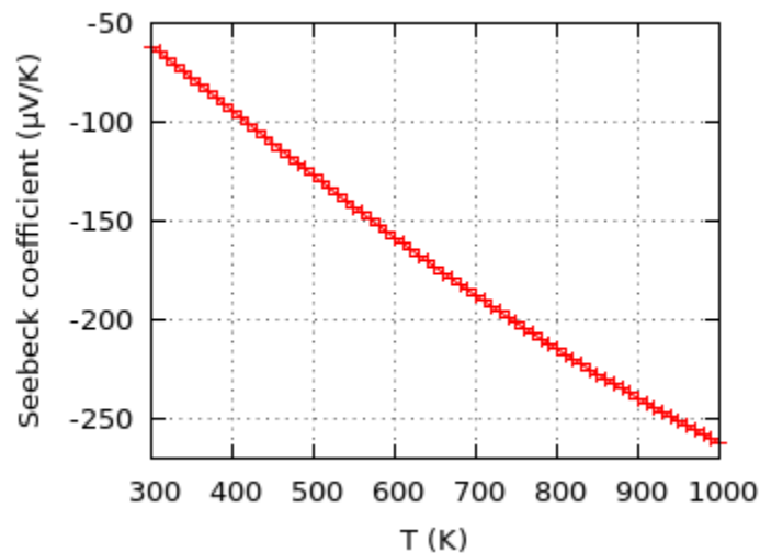
Figure 4: Variation of Seebeck coefficients with temperature.
