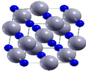
Figure 1.0: (Colour online) The crystal structure of CdO. Where the large grey and small blue balls signify Cd and O respectively.
