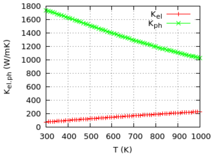
Figure 3: Variation of electronic and lattice contribution of thermal conductivity with respect to temperature.
