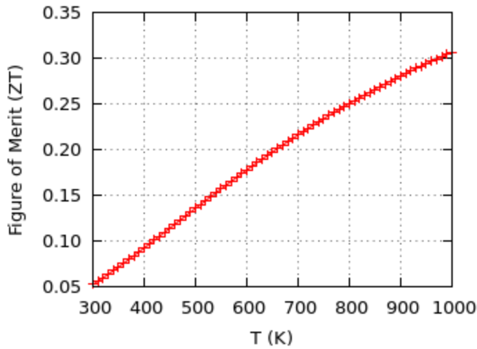
Figure 5: Variation of figure of merit with temperature.
