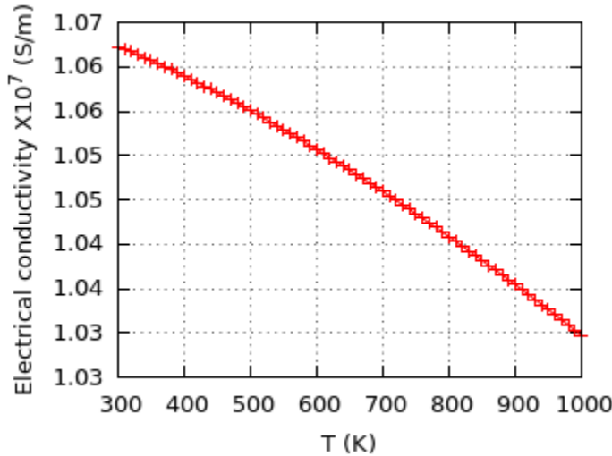
Figure 2: Variation of electrical conductivity with temperature.
