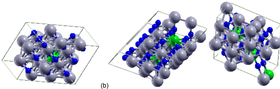
Figure 6: (Colour online) A 3x3x3 supercell of CdO. The large grey and Small blue balls represent Cd and O respectively.
