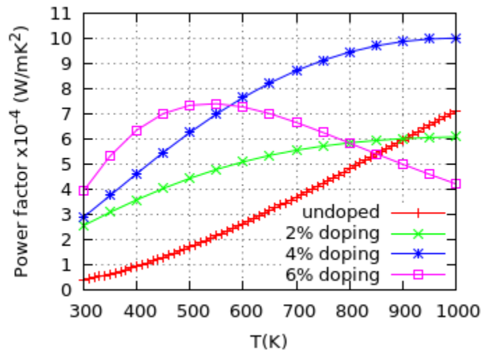
Figure 8: An illustration of the power factor at different concentrations of doping.
