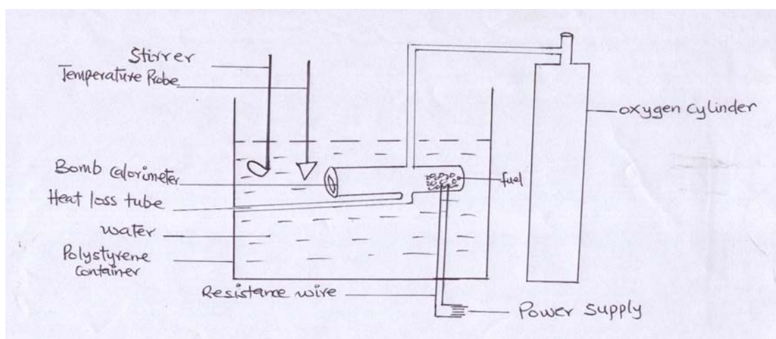
Figure 3: A schematic representation of the experimental set up.
