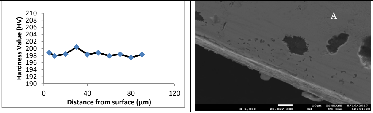
189 Figure 6a: Table showing the correlation between Hardness profiles against SEM micrographs 190 of the un-treated sample 191
