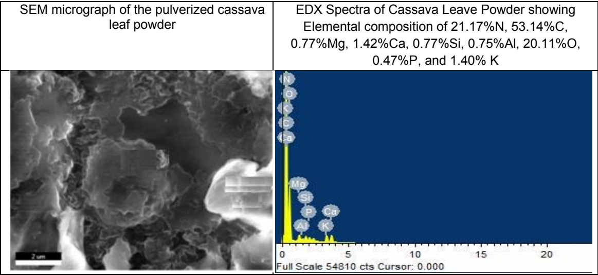
Figure 3: SEM and EDX of the cassava leaf powder
