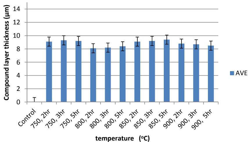
Figure 7: Compound layer and diffusion zone thickness of the pack cyanided cassava leaves samples
