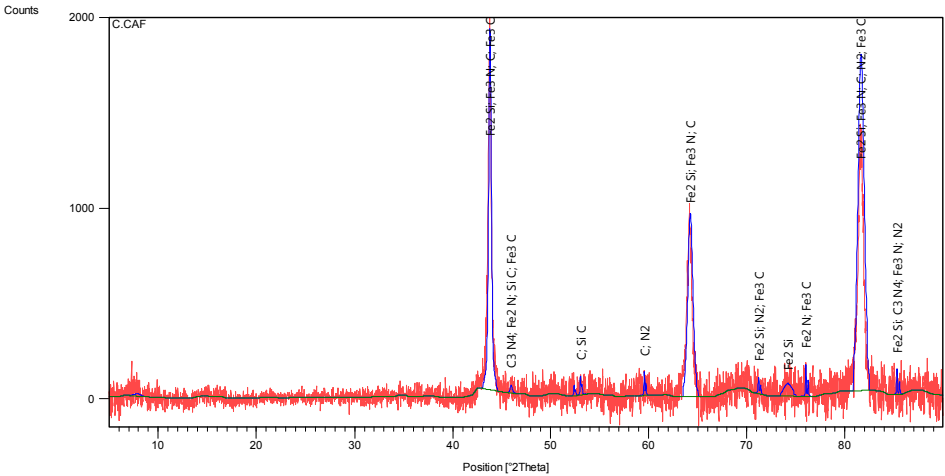
Figure 4a: XRD Pattern of PCCL ductile iron at 850°C for 5 hrs showing intense peak of Fe 3 C, Fe 2 Si, C phases at the core
