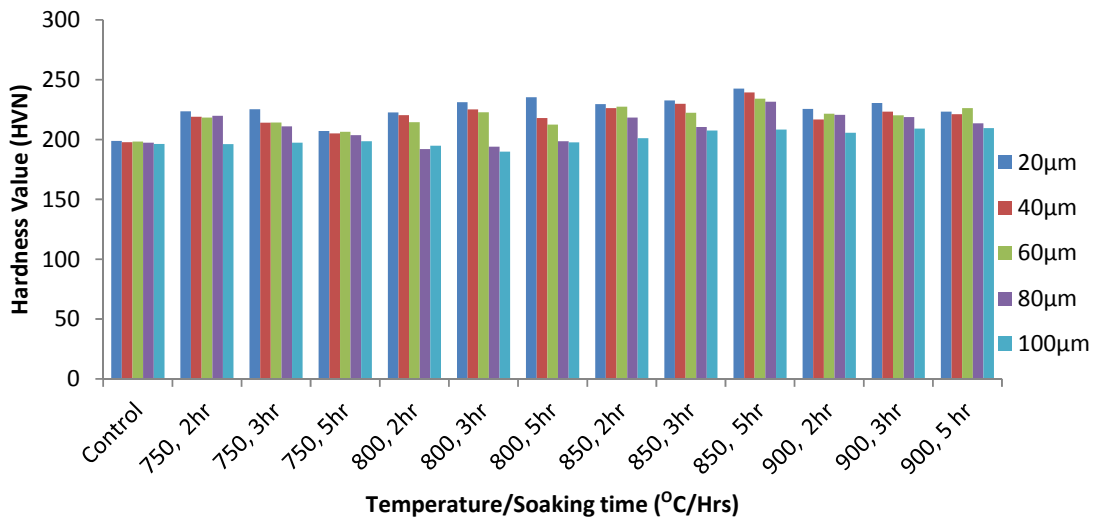
Figure 8: Case hardness with respect to the soaking time for the control and Cassava cyanided Samples
