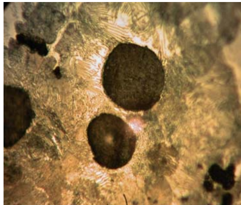
Figure 2: Micrograph of as-cast ductile iron showing graphite nodules and pearlite in a ferrite matrix with free carbide (light irregular particles), 2% nital etched x500.
