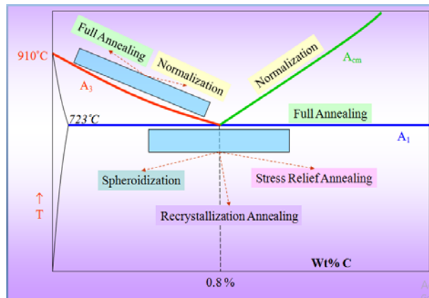
Figure: Comparison of time-temperature cycles for normalizing and full annealing (Romesch, 1993)
