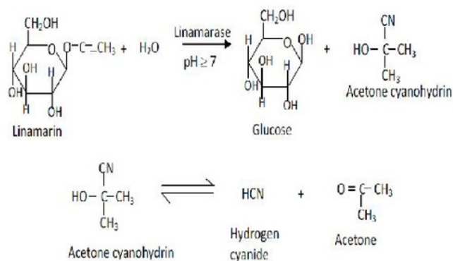
Figure 2: Enzymatic hydrolysis of linamarin (Orijekwe et al. , 2013; Mburu et al. , 2012)
