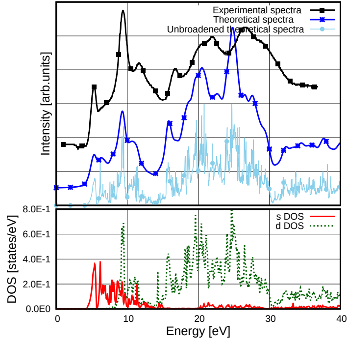
Figure 2: Broadened and unbroadened Mg XANES L_{2,3} edges spectrum calculated using PBE with full core hole compared to the s, d-projected DOS. The experimental spectrum shown was measured by O'Brien et al. [2]
