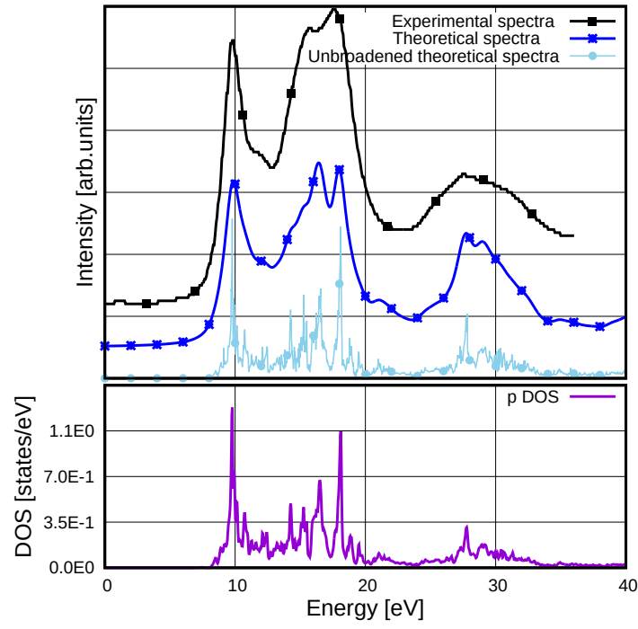
Figure 5: Broadened and unbroadened Mg XANES K edge spectrum calculated using TB-mBJ potential with full core hole compared to the p -projected DOS. The experimental spectrum shown was measured by Luches et al.
