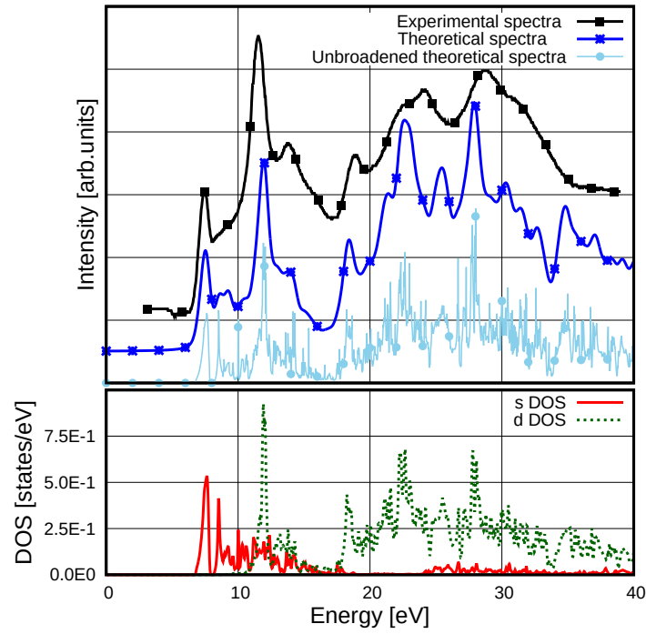
Figure 3: Broadened and unbrodened Mg XANES L_{2,3} edges spectrum calculated using TB-mBJ potential with full core hole compared to the s , d -projected DOS. The experimental spectrum shown was measured by O'Brien et al.
