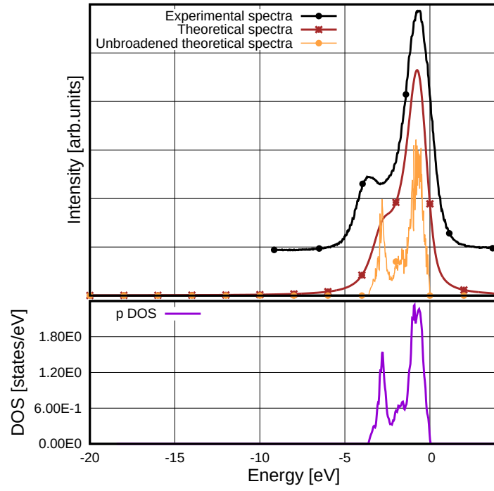
Figure 6: Broadened and unbroadened O K XES spectrum calculated using TB-mBJ potential without core hole in MgO compared to p -projected DOS. The experimental spectrum shown was measured by Galakhov et al. [27]
