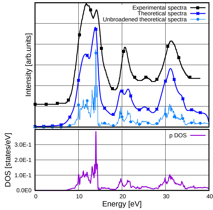
Figure 4: Broadened and unbroadened O XANES K edge spectrum calculated using TB-mBJ potential with full core hole compared to the p -projected DOS. The experimental spectrum shown was measured by Luches et al. [1]
