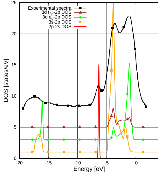
Figure 10: XES Mg L_{2,3} scheme plus 2p \rightarrow 2s extra peak.
