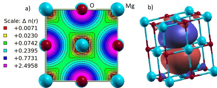
Figure 11: Electronic charge density plot on the (110) plane (a) and the oxygen Wannier function (b).
