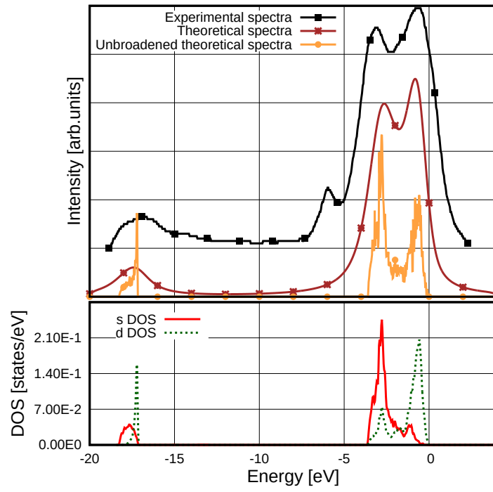
Figure 8: Broadened and unbroadened Mg L_{2,3} XES spectrum compared to s and d -projected DOS calculated using TB-mBJ potential without core hole in MgO. The experimental spectrum was obtained from Ovcharenko et al. [29]
