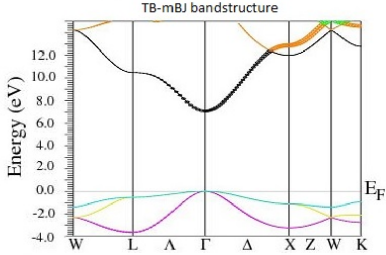
Figure 1: The MgO bandstructure is shown with the increased pick for the s states of Mg atoms. The direct band gap for the \Gamma point is of 7.16 eV.
