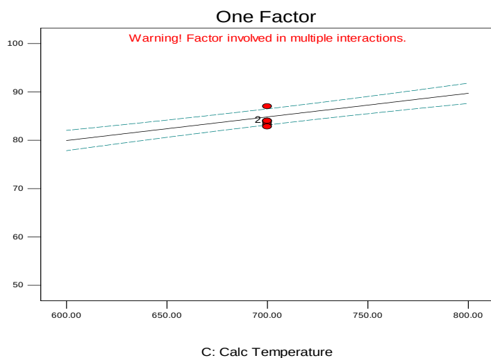
Fig 8c; Effect of Calcination temperature
