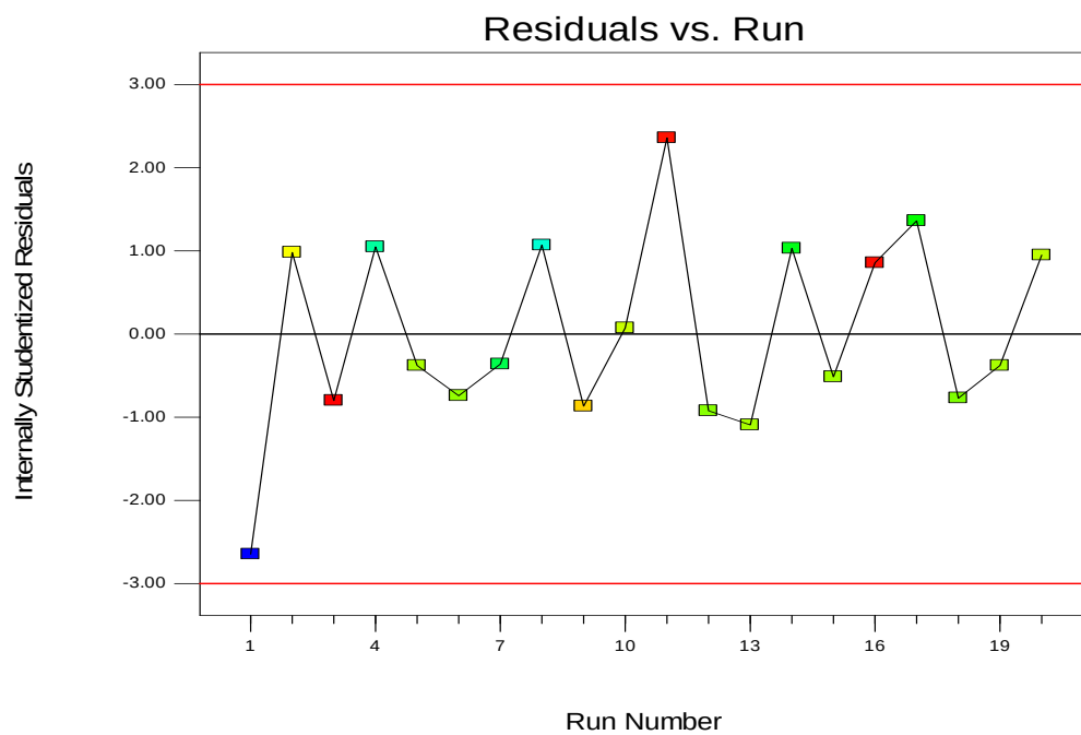
Fig 5: Plot of residuals vs experimental run for zeolite production
