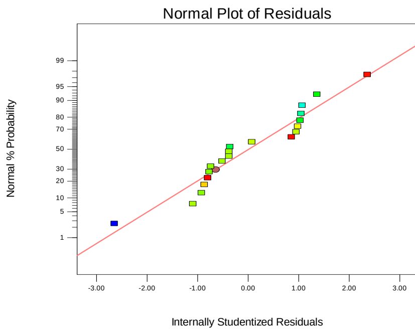
Fig 6: Normal plot of residuals for zeolite production
