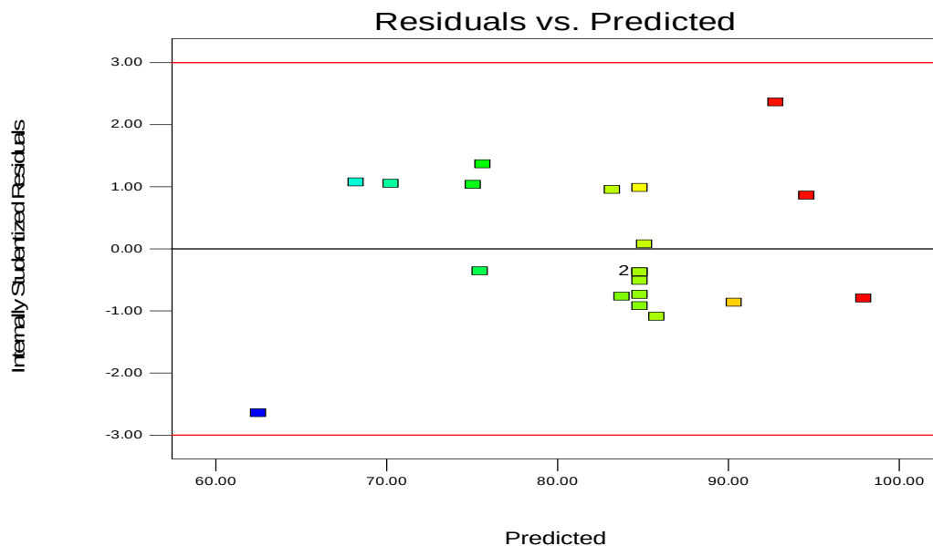
Fig 4: Plot of residual vs predicted for zeolite production
