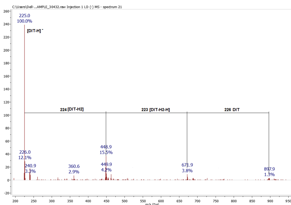
Figure 2. MALDI TOF mass spectrum of complex 5 (colchicine with NaClO 4 ) in the negative ion mode.
