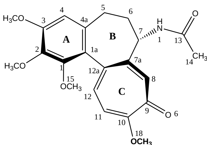
Figure 1. Structure of colchicine 1
