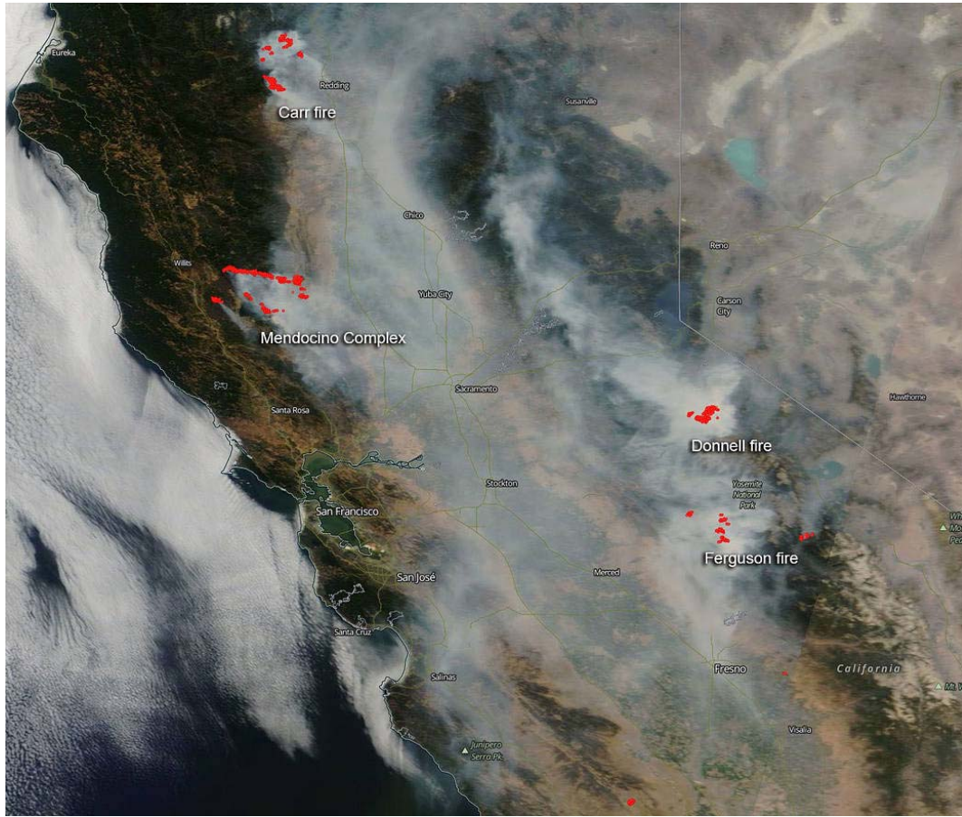
Figure 1. August 7, 2018 NASA image [9] of the California wildfires, the largest in state history [9].
