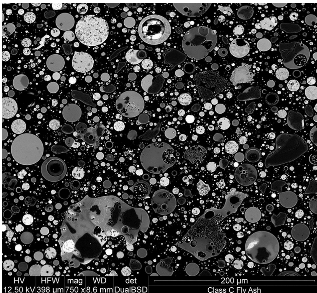
Figure 7. Polished cross section of ASTM C 618 Class C coal fly ash embedded in epoxy. The image was obtained from back-scattered electrons which show differences in atomic density represented by variation in gray scale. Photo courtesy of Wabeggs: CC BY-SA 3.0.
