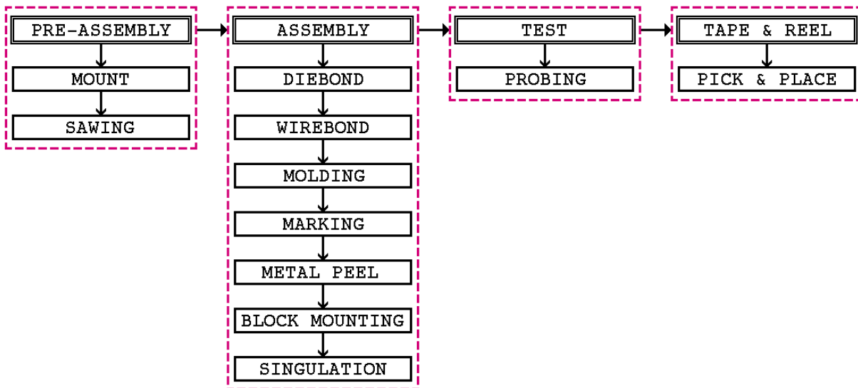
Fig. 3. SPPD complete process flow
