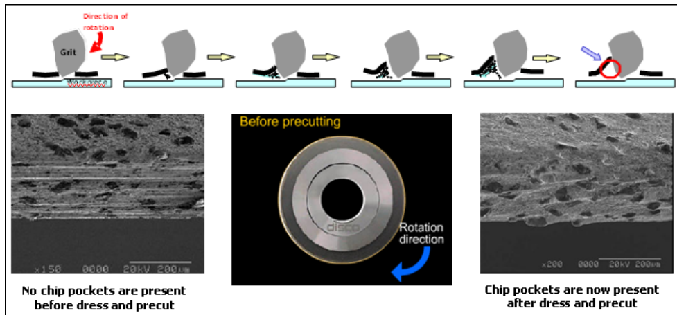
Fig. 8. Dressing and pre-cutting mode
