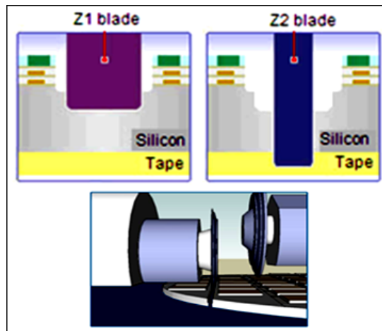
Fig. 9. Step-cutting method
