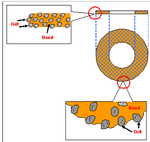
Fig. 7. Elements of blade structure and their purpose
