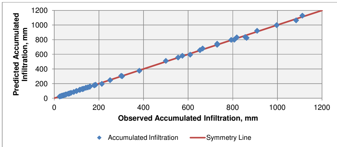
Fig.15. Validation check for the Polynomial infiltration model
