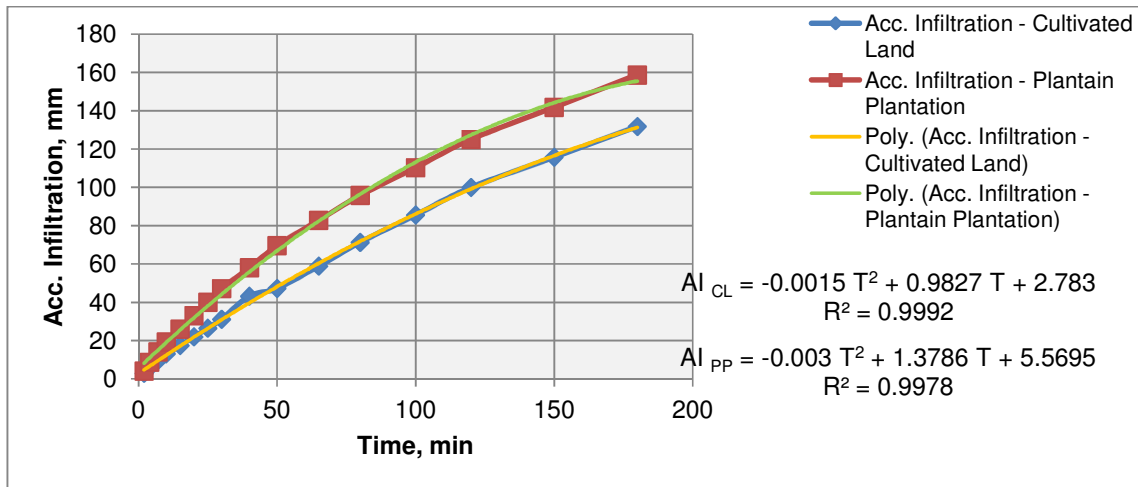
Fig.14. Accumulated infiltration and the obtained equations for other land covers
