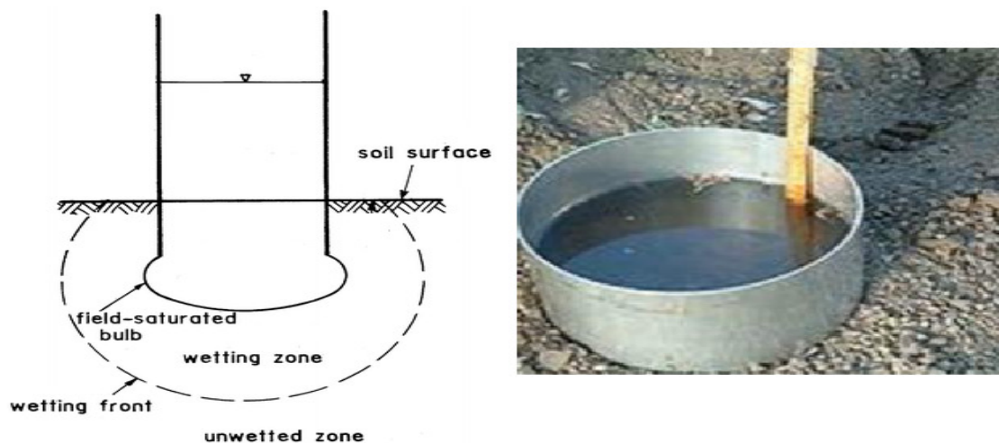
Fig. 2. Single infiltrometer, [8] and [9]
