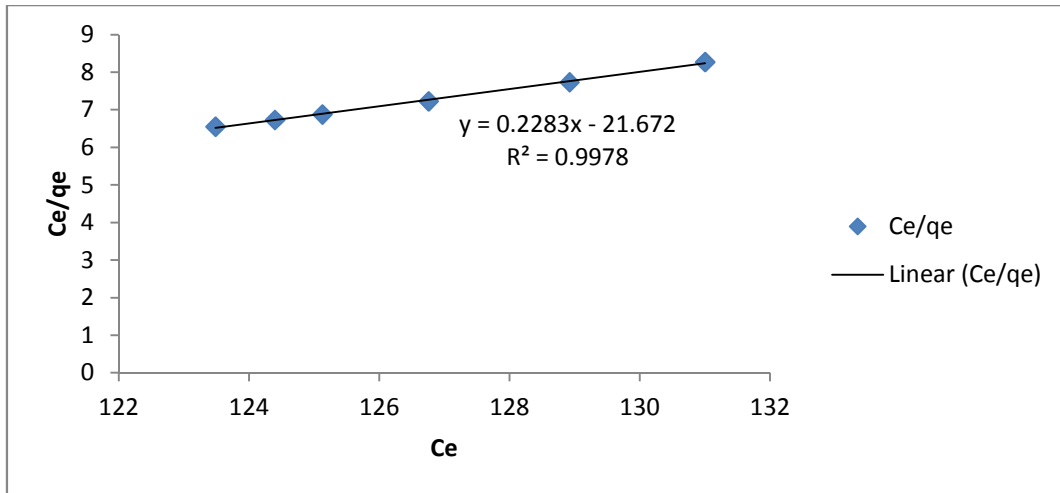
221 222 Figure 3: Composite Langmuir adsorption isotherm plot
