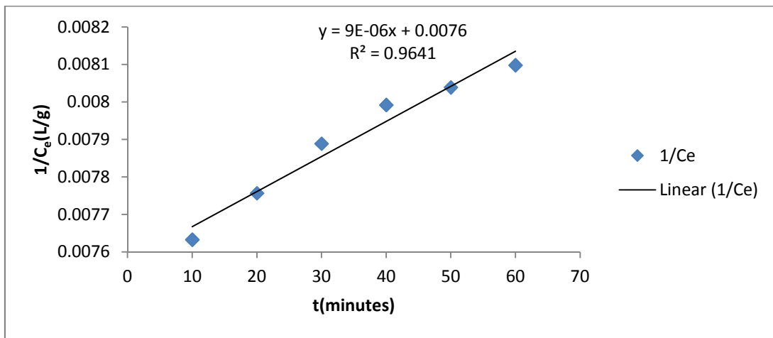
243 244 Figure 7: Composite second order kinetic model
