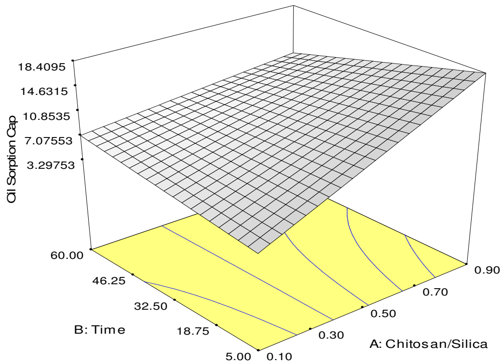
117 118 Figure 1: Response surface 3D plot of OSC versus Contact time and Chitosan/Silica.
