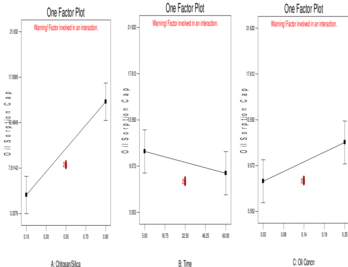
Figure 2: Composite adsorption capacity curve against the variables
