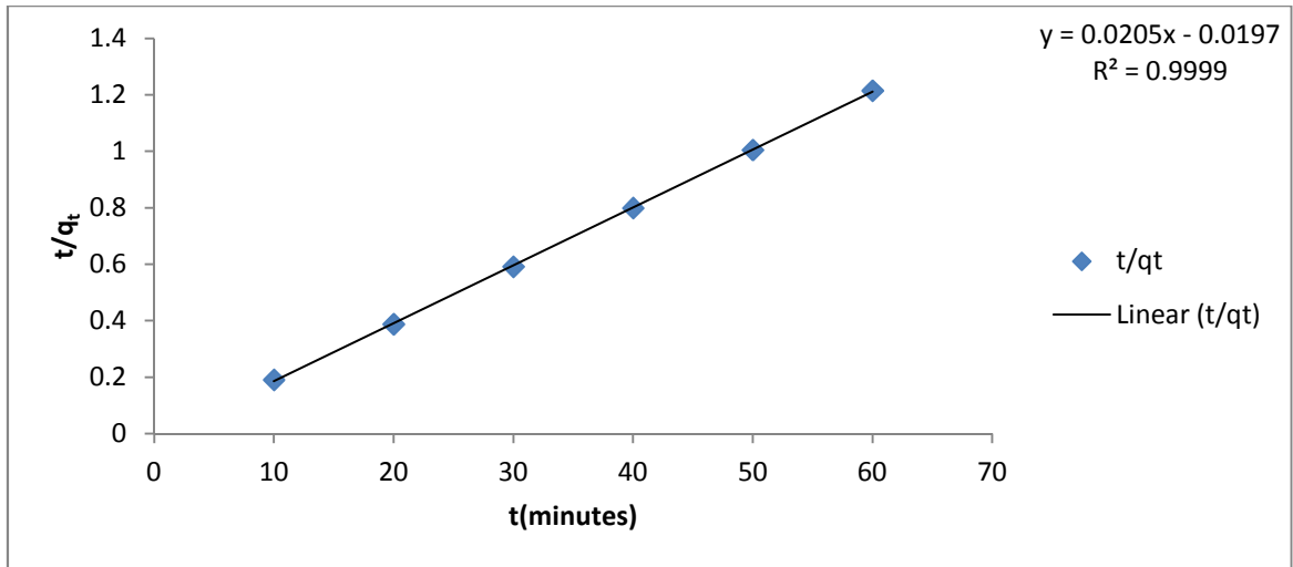
240 241 Figure 6: Composite pseudo-second order kinetic model 242
