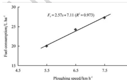
Fig. 1. Tractor fuel consumption as a function of ploughing speed; Adewoyin and Ajav (2013).
