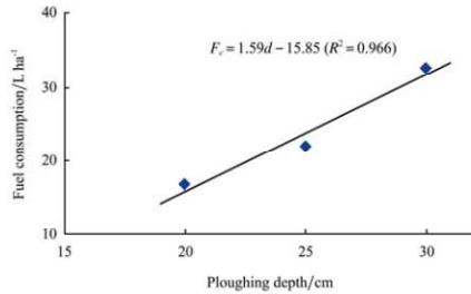
Fig. 3 Tractor fuel consumption as a function of ploughing depth; Adewoyin and Ajav (2013).
