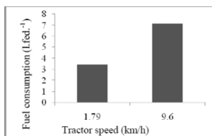
Fig. 2. Effect of tractor speed (km.h -1 ) on fuel consumption (L.fed -1 ); Tayel et al. (2015).
