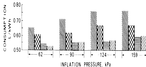
Fig. 6. Effect of inflation pressure on specific fuel consumption with different loads (16, 19, 23 and 26 kN) on the tractor with radial ply tires; Lyne et al. (1984), this figure is a part of the original figure.
