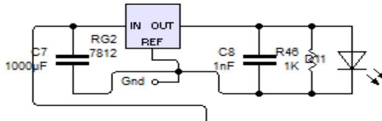
Fig. 8: The inverter on indicator circuit
