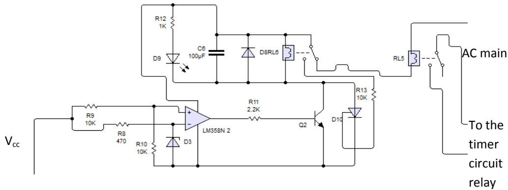
Fig. 4: The battery full circuit
