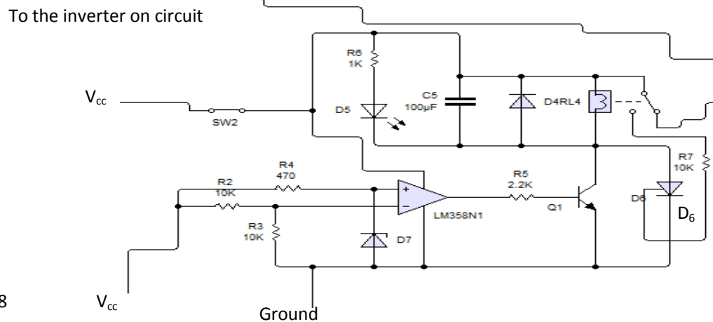
Fig. 3: The battery low circuit
