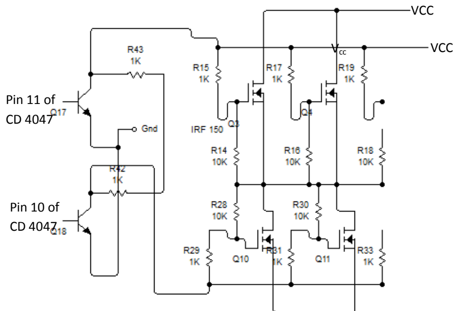
157 Fig. 2: Switching and a section of the current modification circuit
