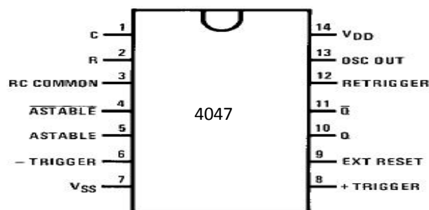
Fig. 7: 4047 Oscillator chip configuration
