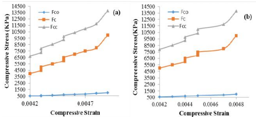
Fig. 11: Graph of Compressive strain against Compressive stress, Tyre pressure and Peak compressive stress: (a) Asphalt Pavement (b) Concrete Pavement
