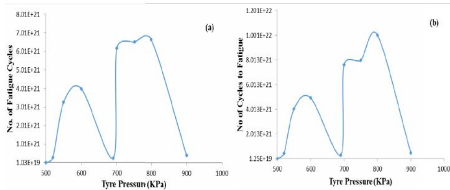
Fig. 14: Graph of layer Tyre Pressure versus No. of cycle to Fatigue under compressive stress at top surface layer for: (a) Asphalt Pavement (b) Concrete Pavement
