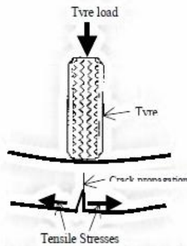
(a) Crack development under wheel load
