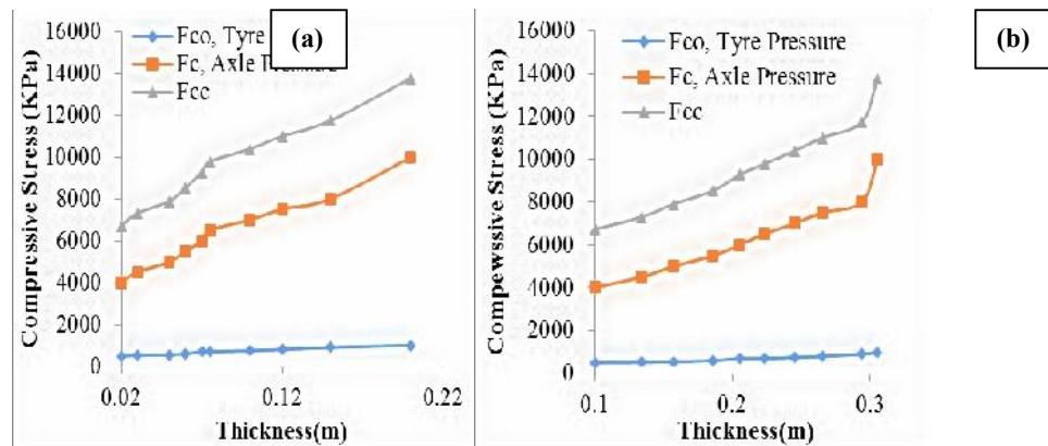
Fig. 5: Graph of layer thickness against Peak compressive stress, Axle pressure and Tyre pressure: (a) Asphalt Pavement (b) Concrete Pavement
