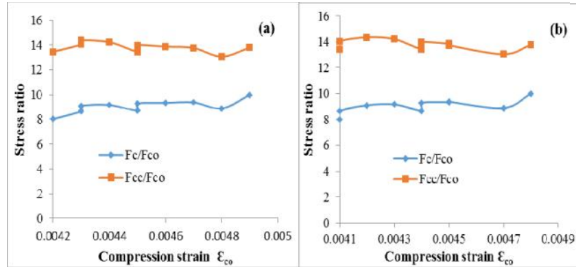
Fig. 9: Graph of Compressive strain against Axial stress and Peak stress ratios: (a) Asphalt Pavement (b) Concrete Pavement
