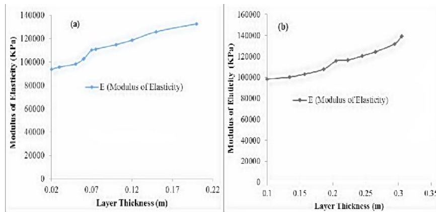
Fig. 7: Graph of layer thickness against Elastic Modulus: (a) Asphalt Pavement (b) Concrete Pavement
