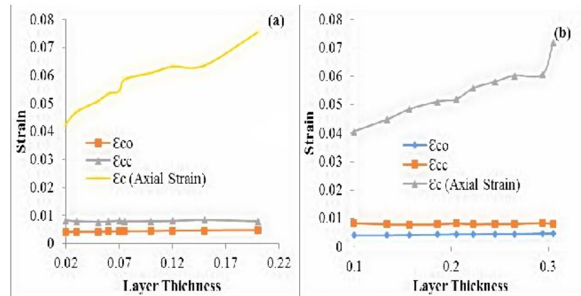
Fig. 6: Graph of layer thickness against Peak compressive strain, Axial strain and Compressive strain: (a) Asphalt Pavement (b) Concrete Pavement
