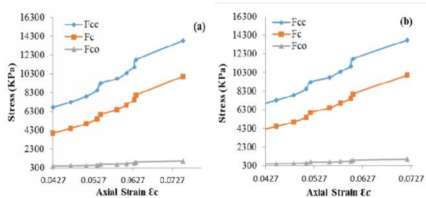
Fig. 10: Graph of Axial strain against Peak compressive stress, Tyre pressure and compressive stresses: (a) Asphalt Pavement (b) Concrete Pavement
