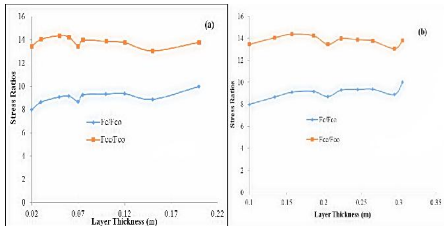
Fig. 8: Graph of layer thickness against Axial stress and Peak Stress ratio (a) Asphalt-Cement Pavement (b) Concrete Cement Pavement
