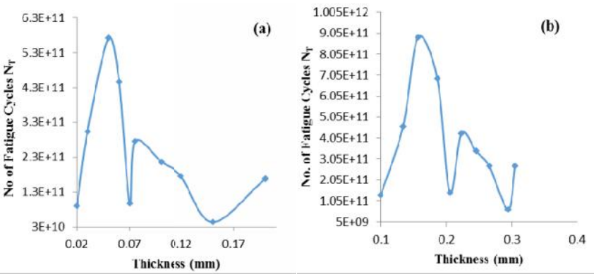
Fig. 13: Graph of layer thickness versus No. of cycle to figure under shear tensile load at Sub-grade level: (a) Asphalt Pavement (b) Concrete Pavement
