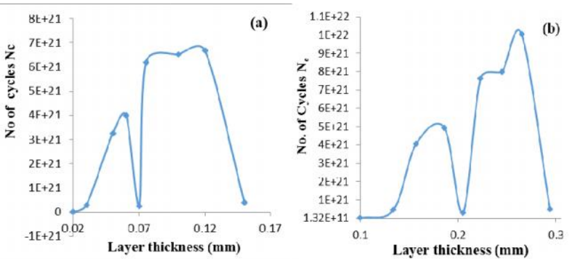
Fig. 12: Graph of layer thickness versus No. of cycle to figure under compression stress at top surface layer: (a) Asphalt Pavement (b) Concrete Pavement
