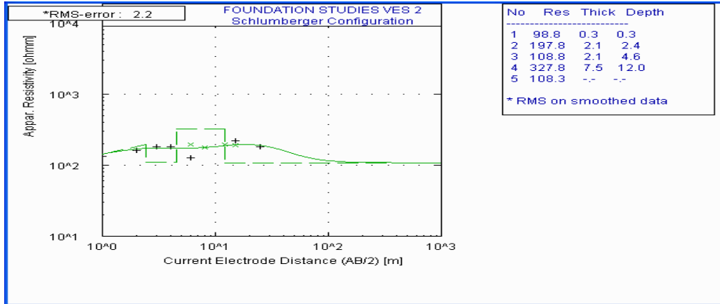
Figure 4e. Typical 'KHK' sounding curve
