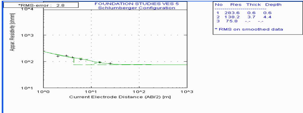
Figure 4d. Typical 'Q' Sounding Curve
