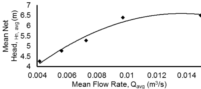
Fig. 7: Mean Net Head and Flow Rate Characteristic for the System
