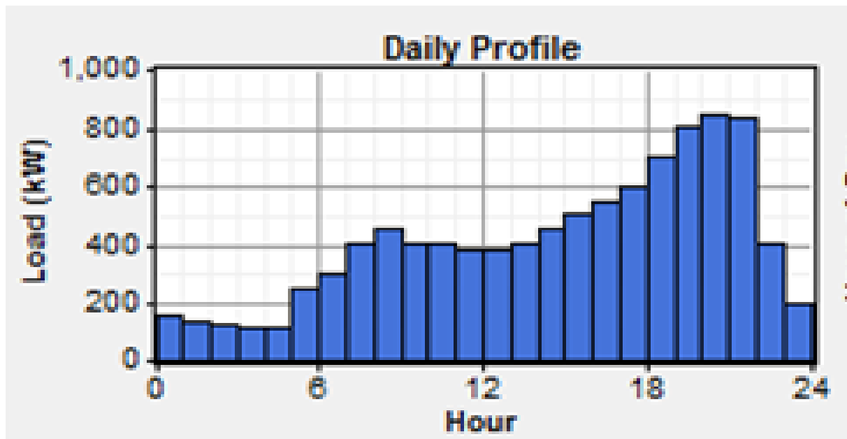
Fig. 4: Hourly load consumption for Erin-Ijesha water fall
