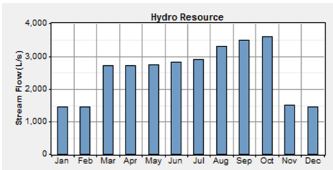
Fig. 5: Hydro resource of Erin-Ijesha water fall (2015)
