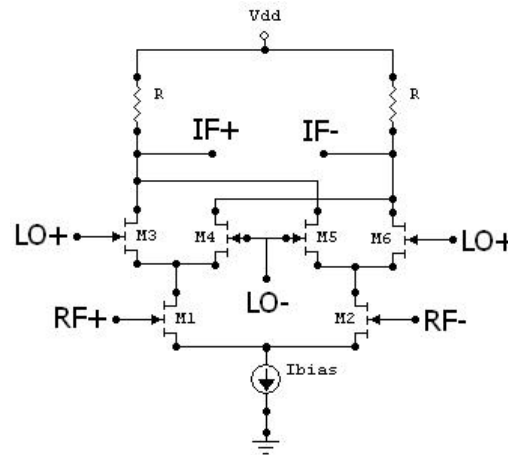
Fig. 3. Double-balanced mixer configuration
