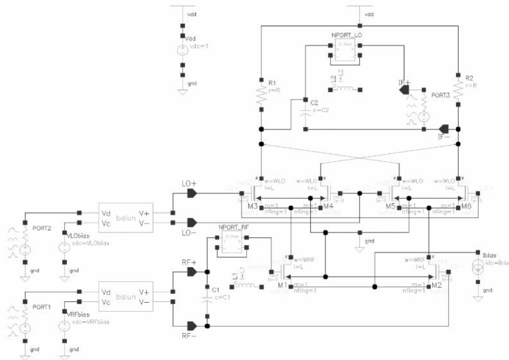
Fig. 4. Schematic design of double-balanced mixer
