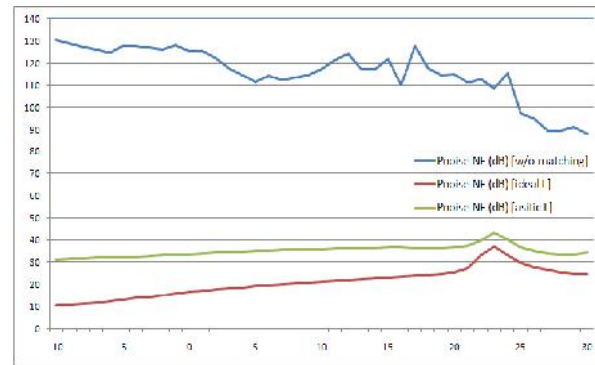
Fig. 8. Noise figure (in dB) vs. P_{LO} of (Pnoise analysis)
