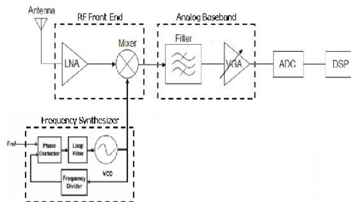
Fig. 1. Block diagram of a typical wireless receiver
