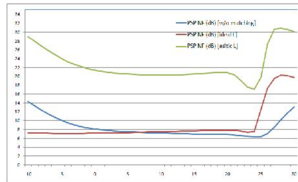
Fig. 9. Noise figure (in dB) vs. P_{LO} of (PSP analysis).
