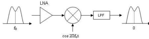
Fig. 2. Direct-conversion or zero-IF receiver
