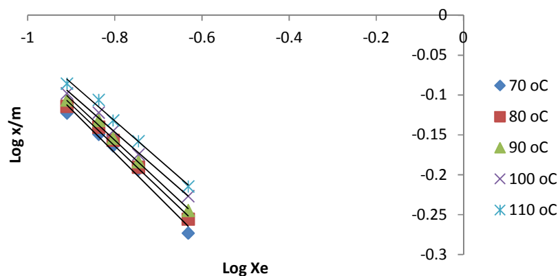
Figure 8: Freundlich Isotherm for the bleaching process
