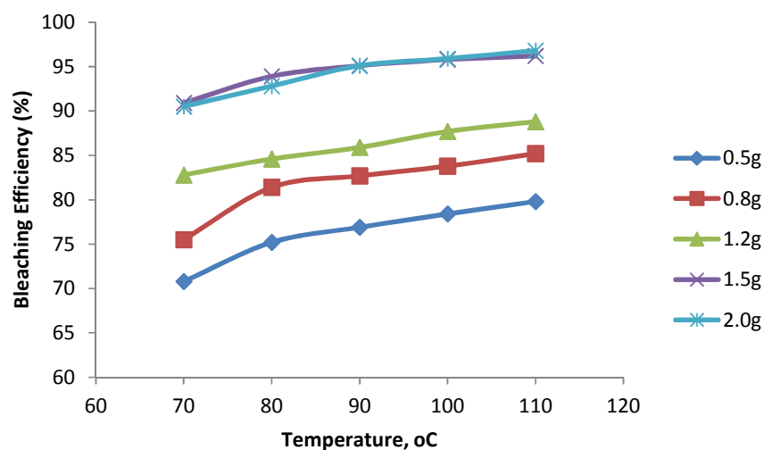
Figure 2: Effect of Temperature and dosage on the bleaching efficiency of Palm oil
