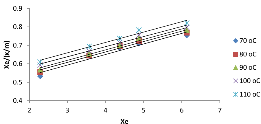
273 Figure 7. Langmuir Isotherm for the bleaching process
