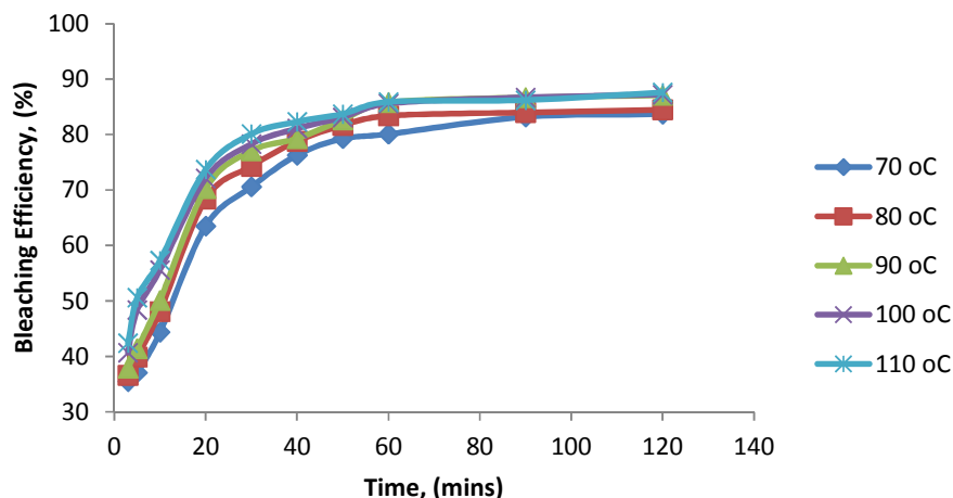
138 Figure 1: Effect of time on the bleaching efficiency of Palm oil
