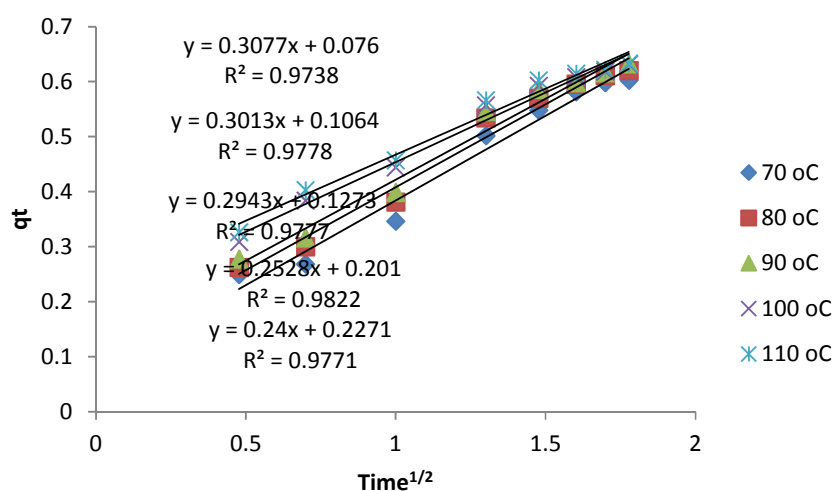
243 Figure 6: Intra particle diffusion kinetic model plot
