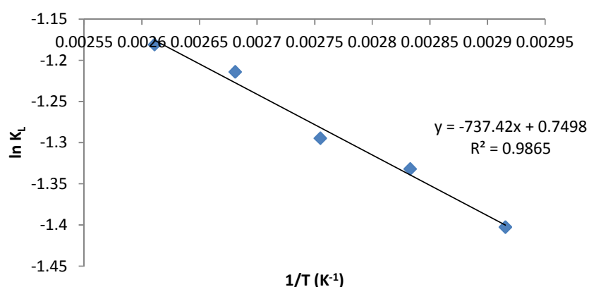
Figure 9: Thermodynamics plot for the bleaching of palm oil
