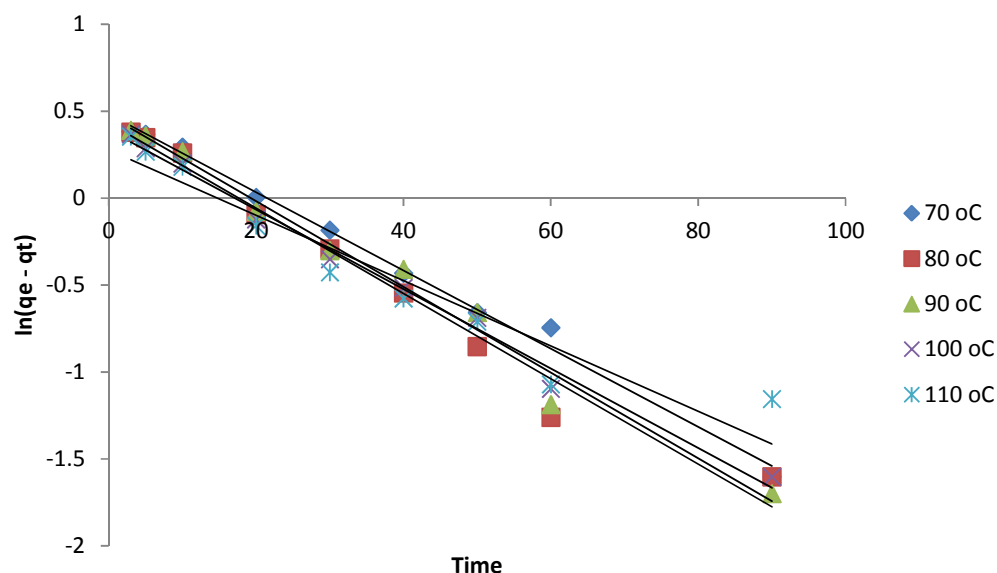
Figure 4: Pseudo First order kinetic plot
