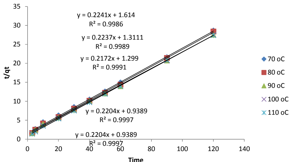
223 Figure 5:Pseudo-second order kinetic model
