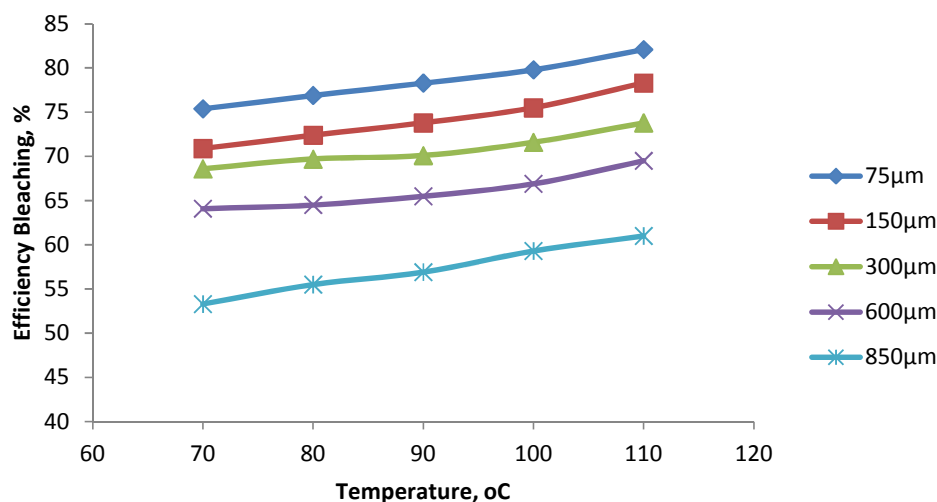
Figure3: Effect of particle size on the bleaching efficiency of Palm oil
