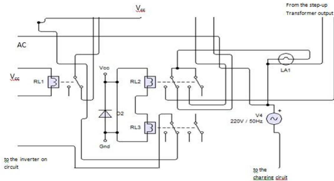
Fig. 5: change-over circuit
