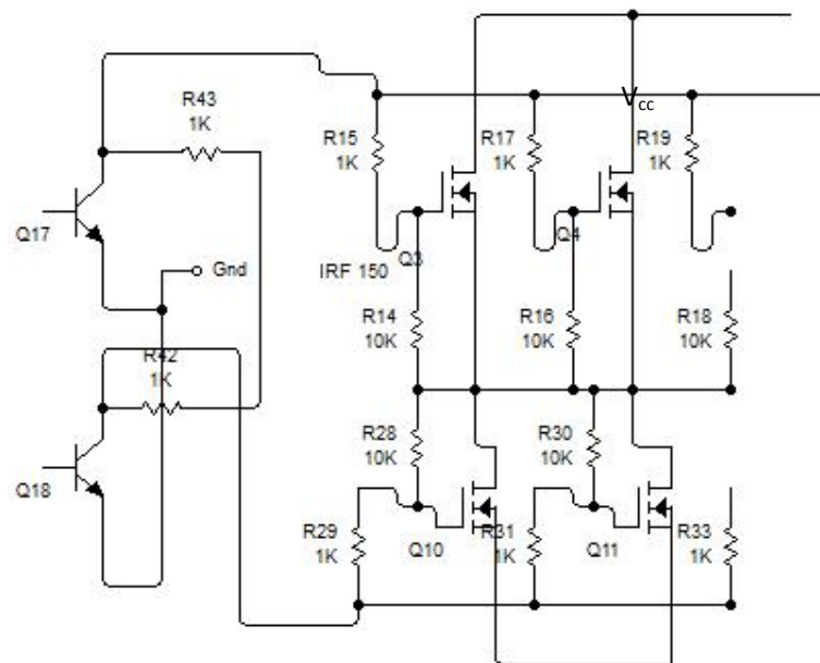
155 Fig. 2: Switching and a section of the current modification circuit
