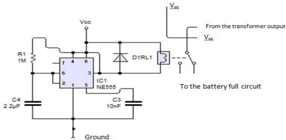
408 Fig.: 9 Delay circuit
