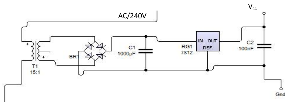
Fig. 6: The Rectifying circuit (Battery charger)
