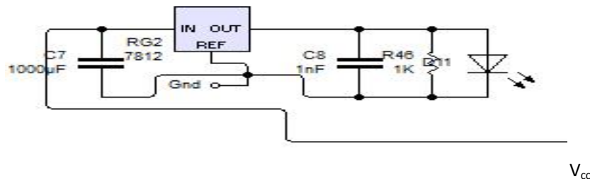
Fig. 8: The inverter on indicator circuit
