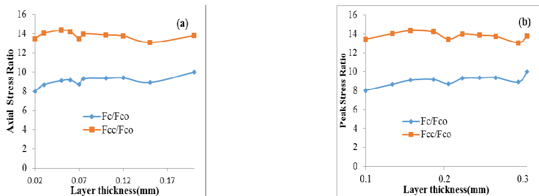
Fig. 8: Graph of layer thickness against axial stress and Peak Stress ratio (a) Asphalt Pavement (b) Concrete Pavement
