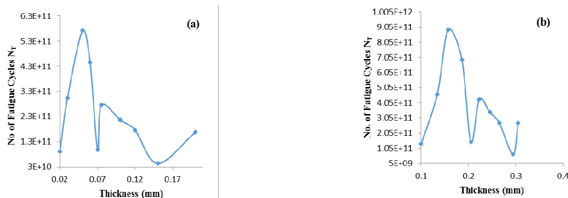
Fig. 13: Graph of layer thickness versus No. of cycle to figure under shear tensile load at Sub-grade level: (a) Asphalt Pavement (b) Concrete Pavement
