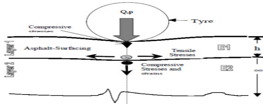
Fig. 3: Simplified Two-Layer Pavement System [1]
