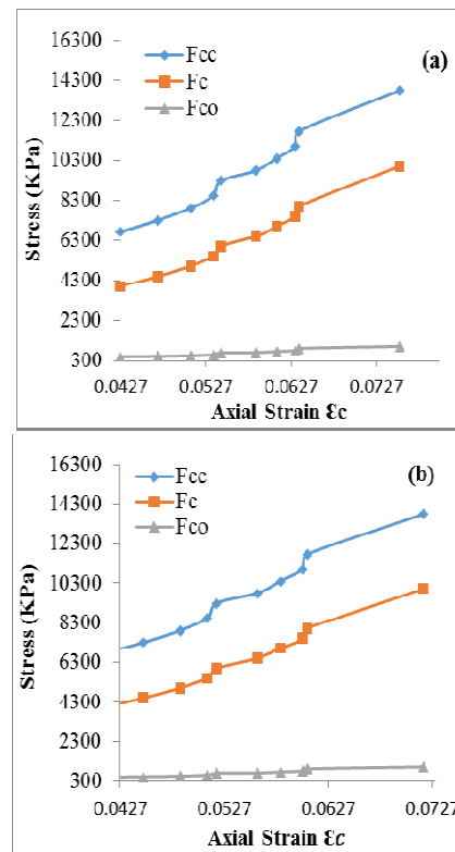
Fig. 10: Graph of Axial strain against Peak compressive stress, Tyre pressure and compressive stresses: (a) Asphalt Pavement (b) Concrete Pavement
