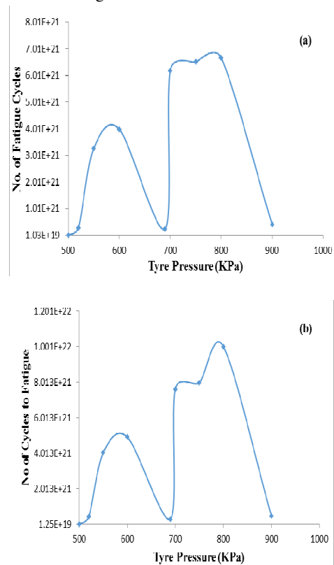
Fig. 14: Graph of layer Tyre Pressure versus No. of cycle to Fatigue under compressive stress at top surface layer for: (a) Asphalt Pavement (b) Concrete Pavement
