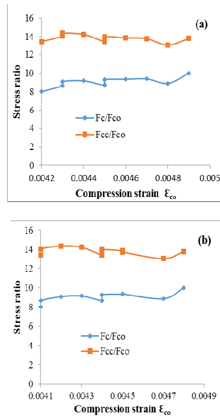
Fig. 9: Graph of Compressive strain against Axial stress and Peak stress ratios: (a) Asphalt Pavement (b) Concrete Pavement
