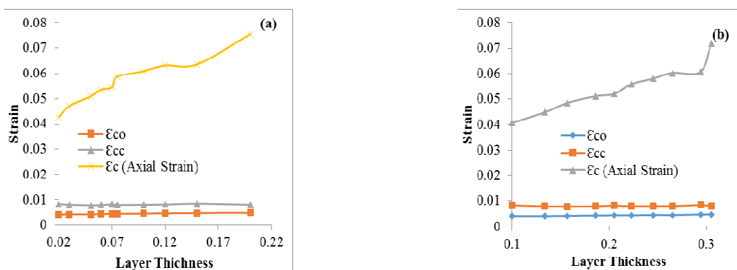
Fig. 6: Graph of layer thickness against Peak compressive strain, Axial strain and Compressive strain: (a) Asphalt Pavement (b) Concrete Pavement
