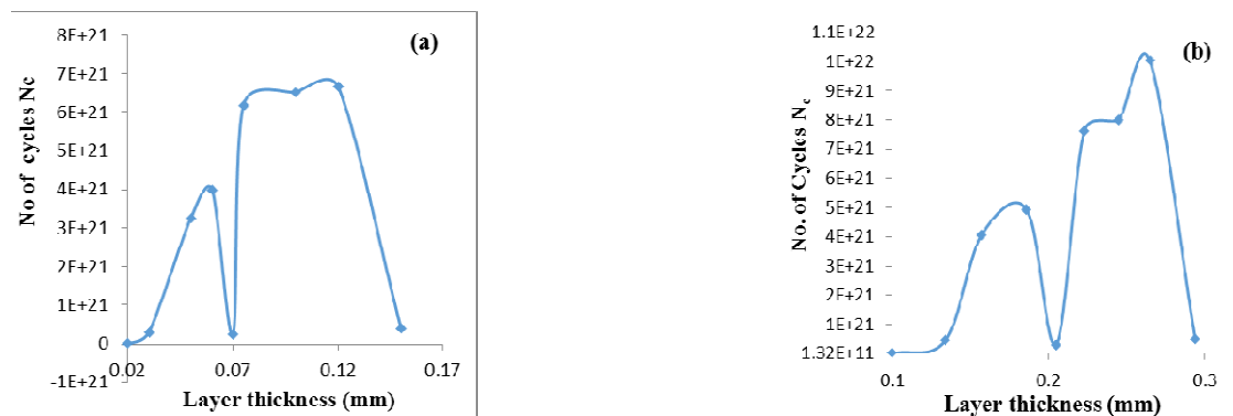
Fig. 12: Graph of layer thickness versus No. of cycle to figure under compression stress at top surface layer: (a) Asphalt Pavement (b) Concrete Pavement
