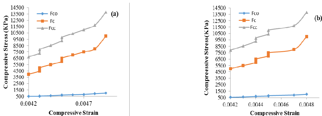
Fig. 11: Graph of Compressive strain against Compressive stress, Tyre pressure and Peak compressive stress: (a) Asphalt Pavement (b) Concrete Pavement
