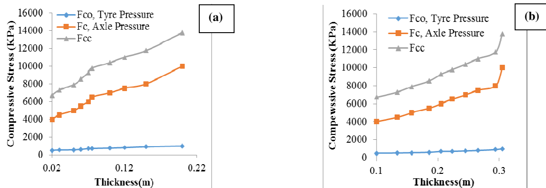
Fig. 5: Graph of layer thickness against Peak compressive stress, Axle pressure and Tyre pressure: (a) Asphalt Pavement (b) Concrete Pavement
