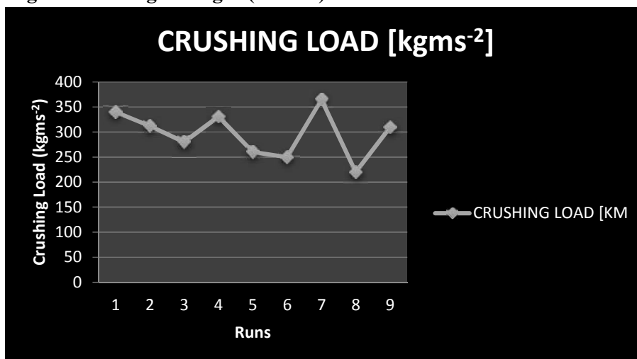
232 Fig 3: Crushing Load [\text{kgms}^{-2}] Result for Crushed Concrete Cubes at Seven Days
