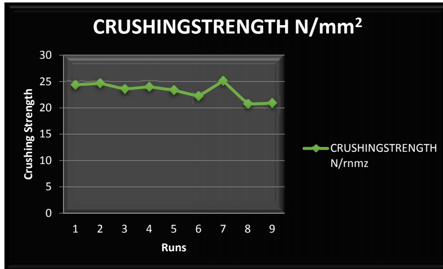
257 Fig 9: Crushing Strength [N/mm 2 ] Result for Crushed Concrete Cubes at Twenty Eight 258 Days
