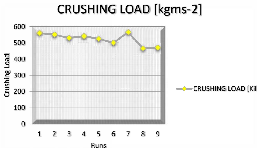
261 Fig 10:Crushing Load [kgms -2 ] Result for Crushed Concrete Cubes at Twenty Eight Days
