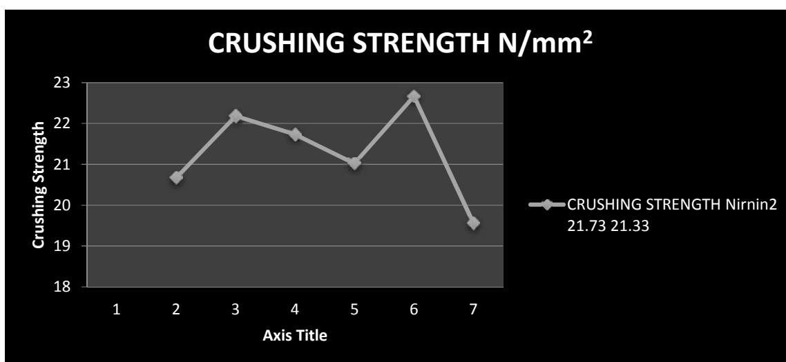
230 Fig 2: Crushing Strength ( \text{N/mm}^2 ) Result for Crushed Concrete Cubes at Seven Days
