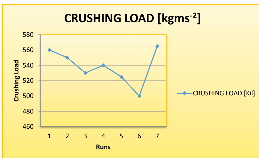
251 252 Fig 8: Crushing Load [kgms -2 ] Result for Crushed Concrete Cubes at Twenty one Days 253
