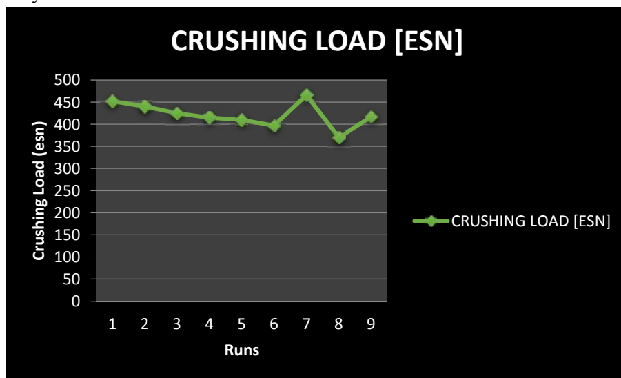
242 243 Fig 6: Crushing Load [ESN] Result for Crushed Concrete Cubes at Fourteen Days
