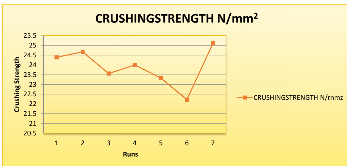
248 249 Fig 7: Crushing Strength [N/mm 2 ] Result for Crushed Concrete Cubes at Twenty one 250 Days
