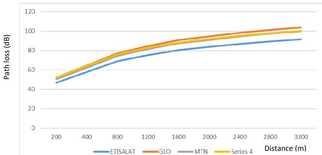
Figure 6: Path loss outside building B3, from the generated models for Etisalat, Glo, MTN and log distance n=4
