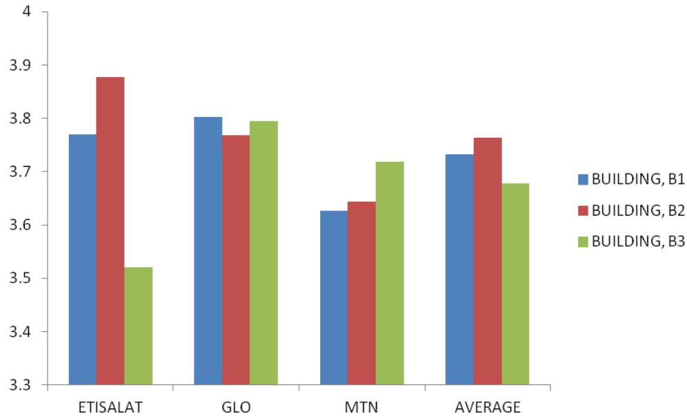
Figure3: Penetration loss of the three buildings under study
