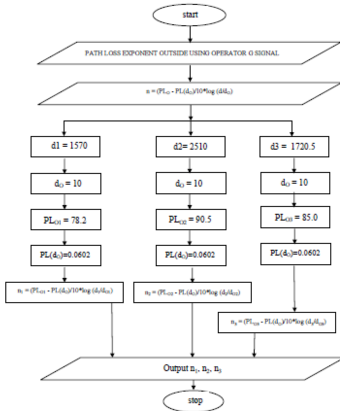
Figure A4: Flow Chart for Computing the Path Loss Exponent of Buildings B1, B2, B3 using Operator G Signals
