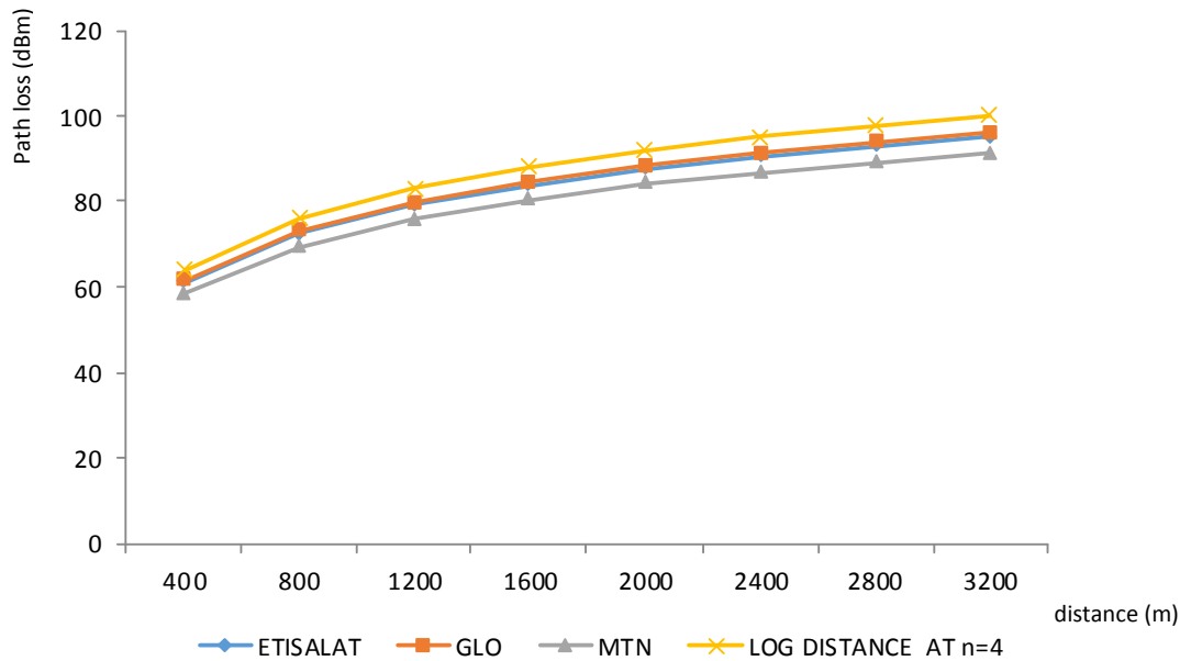
Figure4: Path loss outside building B1, from the generated models for Etisalat, Glo, MTN and log distance n=4
