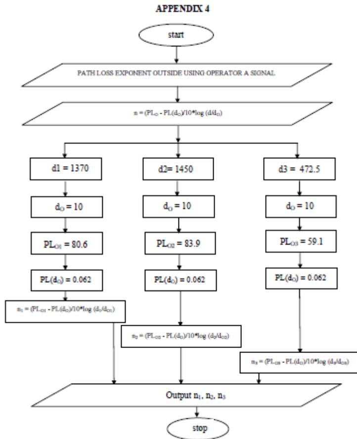
Figure A3: Flow Chart for Computing the Path Loss Exponent of Buildings B1, B2, B3 using Operator A Signals
