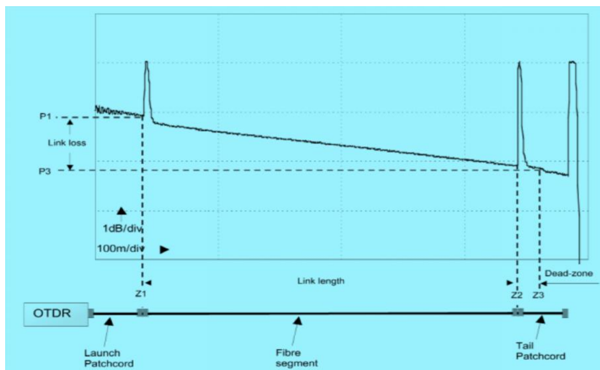
Figure 2: OTDR Trace
