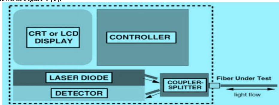
Figure 1: OTDR block diagram
