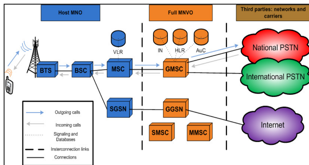
Figure 1: Full MNVO – Backbone
