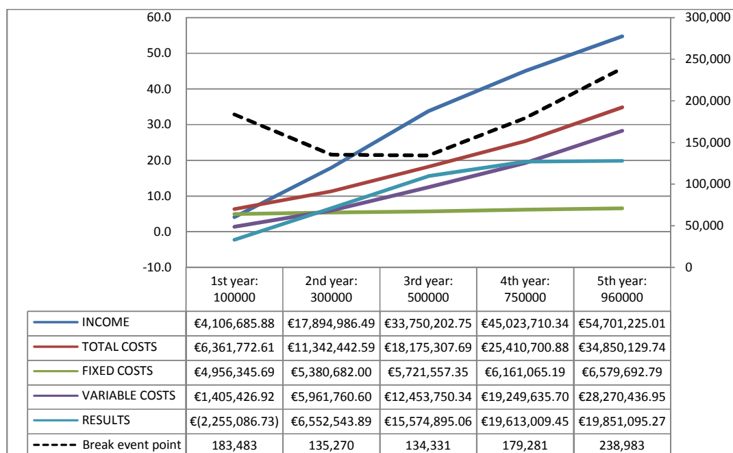
Figure 9: Total income, total costs and break-even point for scenario 3-a
