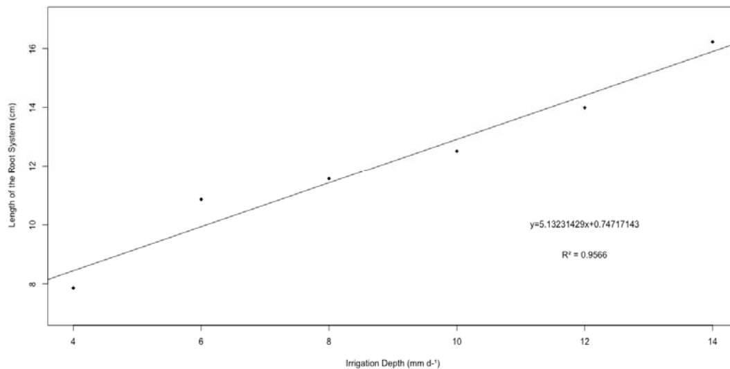
Fig. 4. Variation of root system length under different irrigation depths in papaya seedlings
