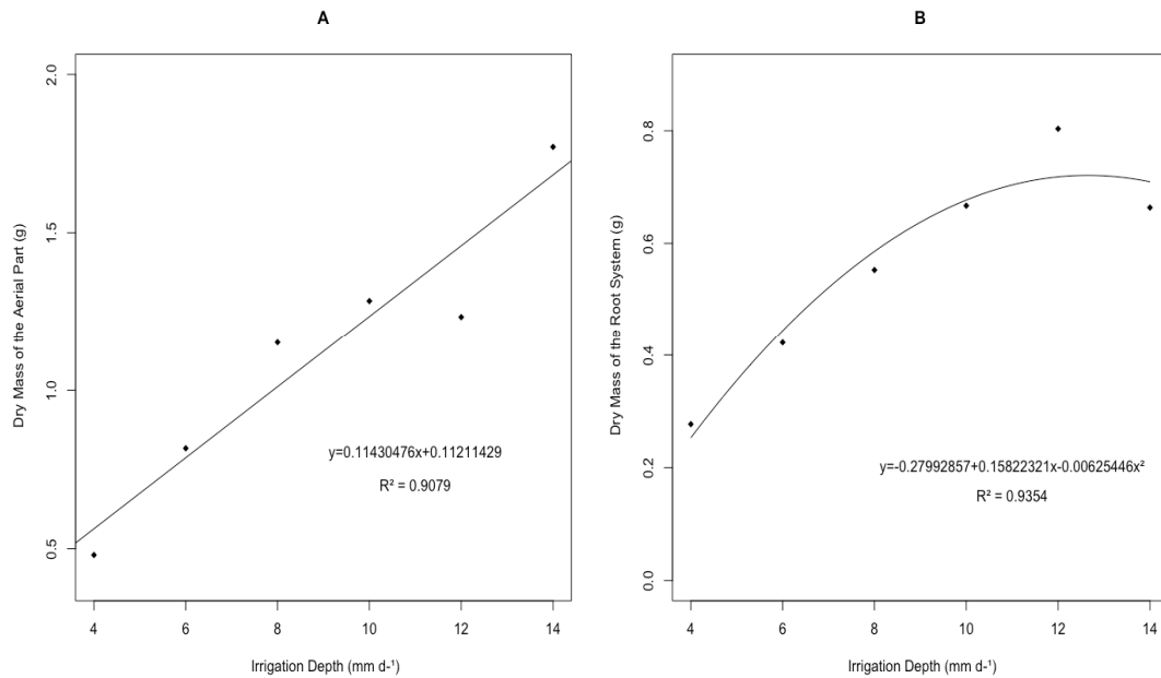
Fig. 7. Variation of the dry mass of the aerial part (A) and the dry mass of the root system (B) of papaya seedlings, under different irrigation depths
