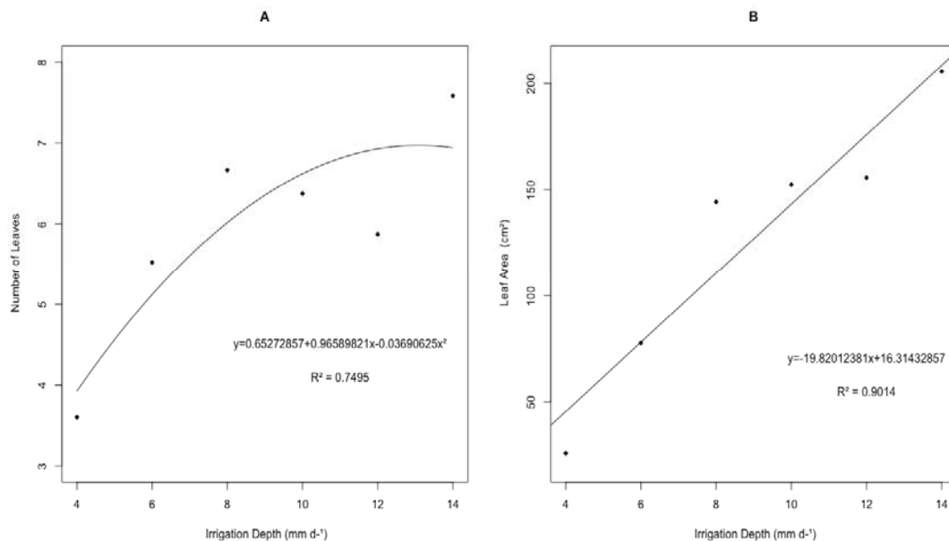
182 Fig. 5. Variation of number of leaves (A) and leaf area (B), under different 183 irrigation depths in papaya seedlings
