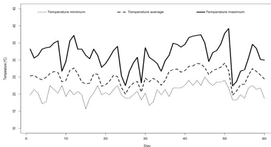
Fig. 1. Average, maximum and minimum temperatures during the experiment period in Colatina, Espírito Santo
