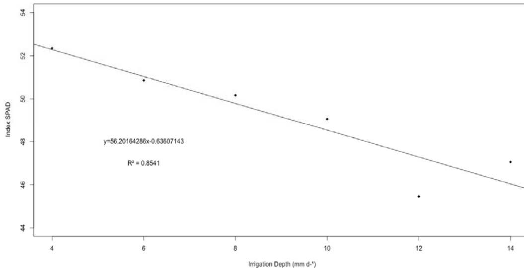
201 Fig. 6. Variation of the SPAD index, under different irrigation depths in papaya 202 seedlings
