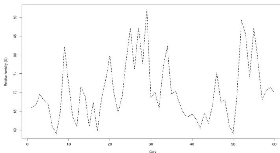
Fig. 2. Average relative humidity during the experiment period in Colatina, Espírito Santo
