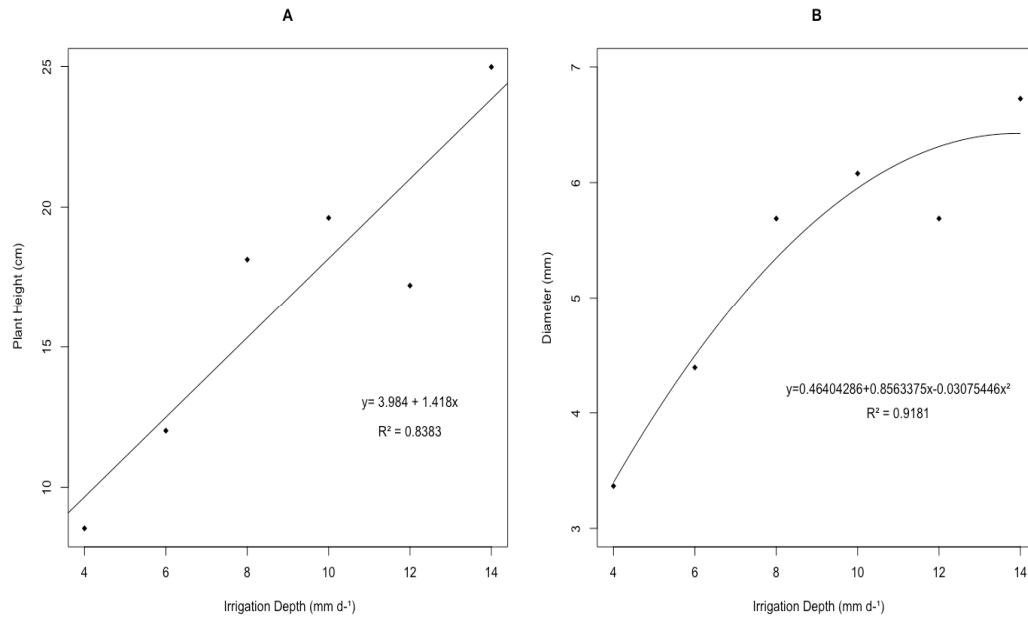
Fig. 3. Variation of plant height (A) and stem diameter (B), under different irrigation depths in papaya seedlings
