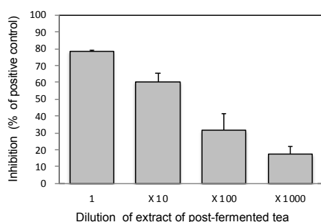
Fig. 3. Inhibitory effect of the infusion of post-fermented green tea with reduced caffeine on adipogenesis. Each bar shows the mean \pm SEM (n=3).
