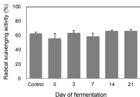
Fig. 2. Anti-oxidative activity of the infusion of post-fermented green tea with reduced caffeine. DPPH radical scavenging activity was analyzed spectrophotometrically. Each bar shows the mean \pm SEM (n=3).
