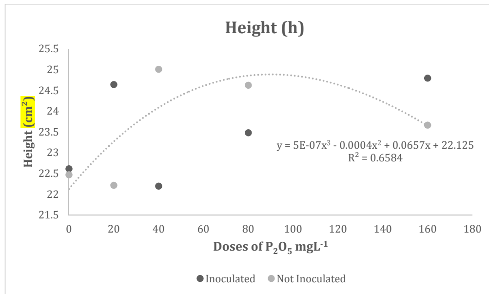
176 Fig. 1 Height (h) of Parkia nitida seedlings as a function of arbuscular mycorrhizal fungi (FMA) 177 and phosphate fertilization, 153 days after transplanting
