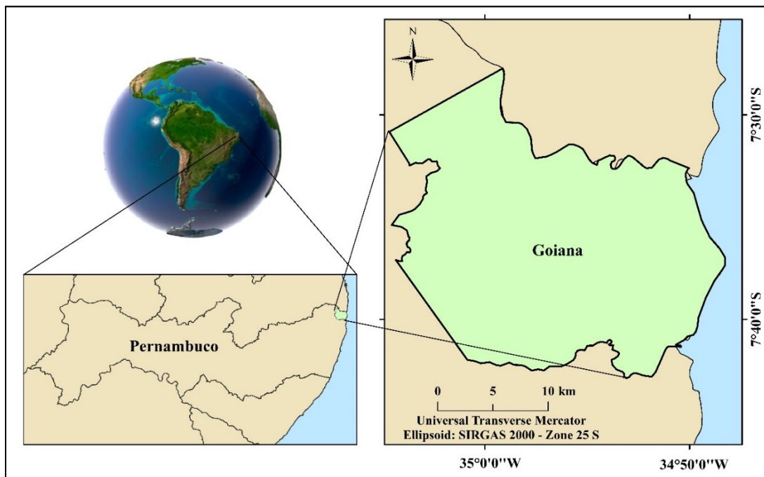
99 Fig. 1. Location of the study area in the municipality of Goiana, PE, Brazil, 2017.
