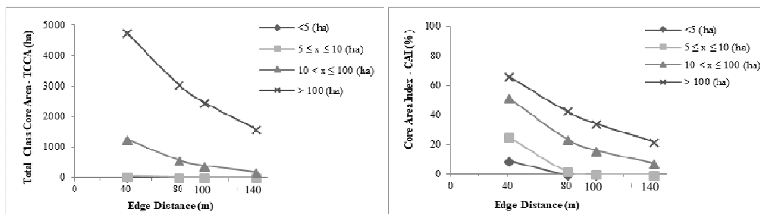
Fig. 3. Behavior of the total class core area and the core area index with the increase of edge distance in the size classes of native vegetation fragments in the municipality of Goiana, PE, Brazil.
