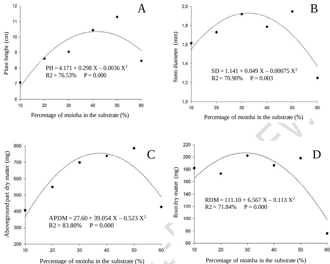
Figure 3. Plant height (A), stem diameter (B), aboveground part dry matter (C) and root dry matter (D) as a function of different percentage of moinha in the substrate (treatments).
