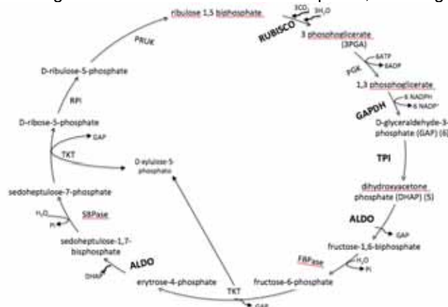
Figure 5. The Calvin cycle. Abundant proteins in normal banana plants are shown in bold letters. Enzymes encoded by non-differentially expressed genes are shown with normal letters. Abbreviations for enzymes: ALDO: aldolase (fructose-bisphosphate aldolase); FBPase: fructose-1,6-bisphosphatase; GAPDH: glyceraldehyde-3-phosphate dehydrogenase; PGK: phospho-glycerate kinase; PRUK: phosphoribulokinase; RPE, ribulosephosphate 3-epimerase; RPI: ribose 5-phosphate isomerase; Rubisco: ribulose-1,5-bisphosphate carboxylase/oxygenase; SBPase: sedoheptulose-1,7-bisphosphatase; TKT: transketolase; TPI: triose-phosphate isomerase.
