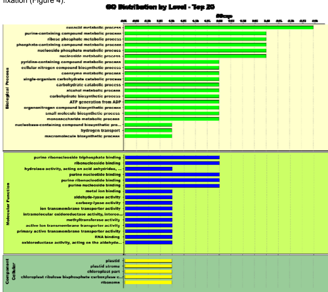
230 Figure 4. The Blast2GO results are summarized into three main GO categories: biological 231 process (BP), cellular component (CC), and molecular function (MF). Only the top ten GO 232 terms for each main function category are shown (green: BP; blue: MF; yellow: CC). 233
