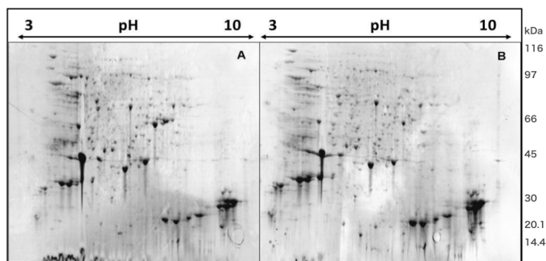
211 212 Figure 3. 2-DE gels for both normal banana leaf (A) and giant plant leaf (B) samples. 213
