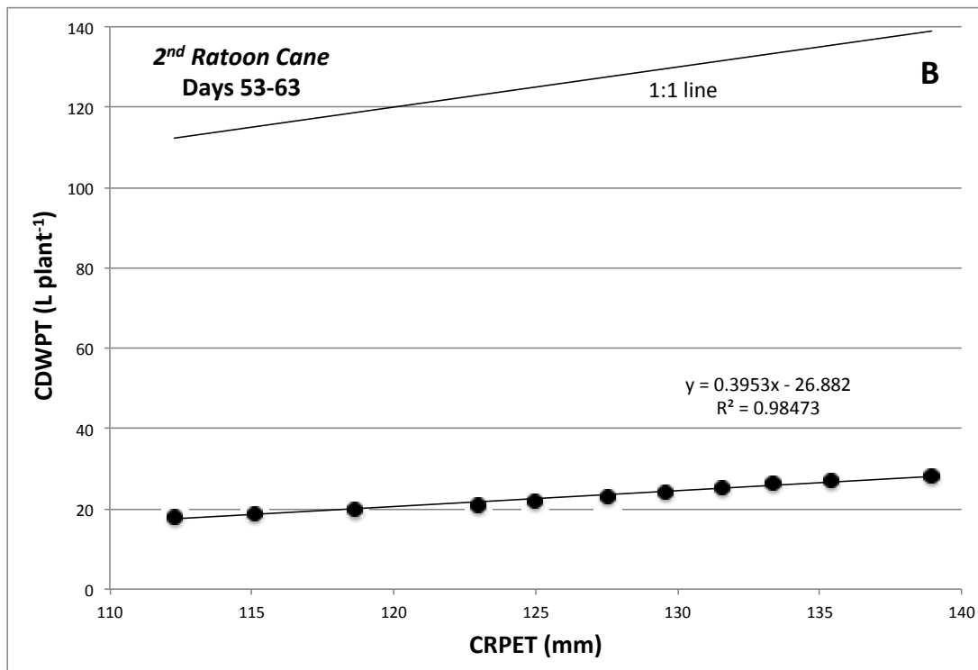
Figure 7. Linear regression of cumulative whole-plant transpiration (CDWPT) on cumulative reference potential evapotranspiration (CRPET) calculated for distinct periods within the second ratoon cane phase of the study: 1 to 52 days (A) and 53 to
