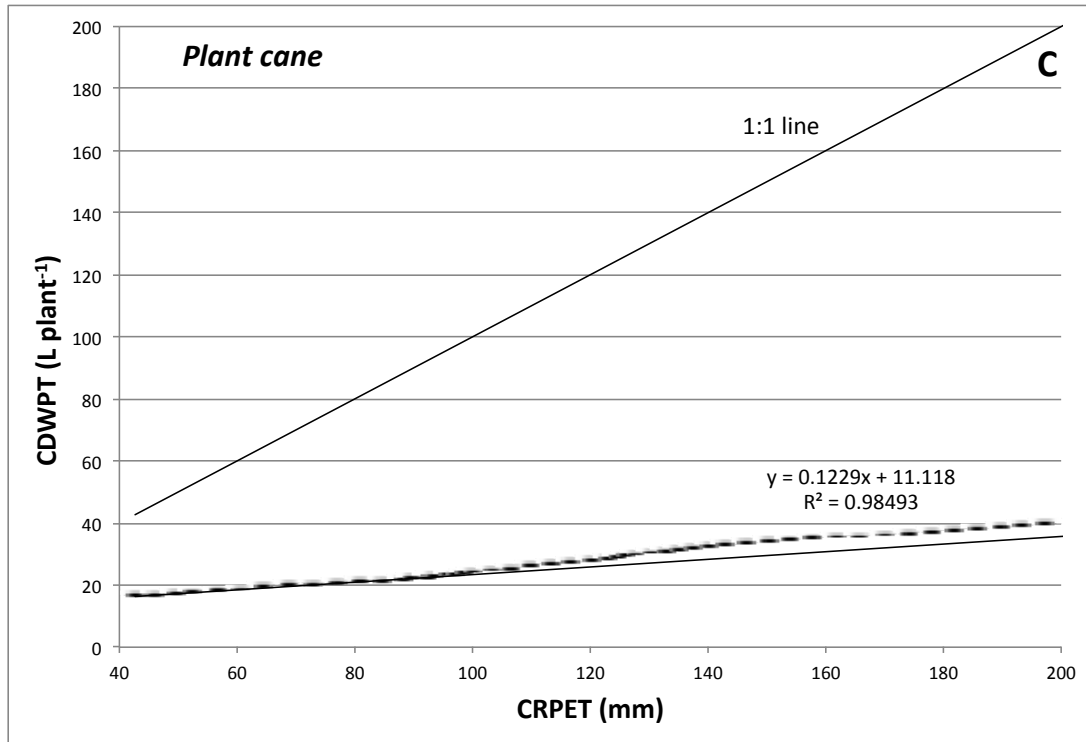
Figure 3. Linear regression of cumulative whole-plant transpiration (CDWPT) on cumulative reference potential evapotranspiration (CRPET) calculated for distinct periods within the plant cane phase of the study: 1 to 10 days (A), 11 to 20 days (B), and 21 to 99 days (C). Cumulative whole-plant transpiration values were calculated with daily whole-plant transpiration averaged across the three studied genotypes.
