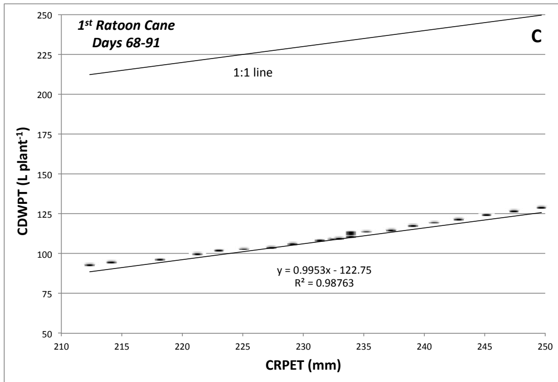
Figure 5. Linear regression of cumulative whole-plant transpiration (CDWPT) on cumulative reference potential evapotranspiration (CRPET) calculated for distinct periods within the first ratoon cane phase of the study: 1 to 20 days (A), 21 to 67 days (B), and 68 to 91 days (C). Cumulative whole-plant transpiration values were calculated with daily whole-plant transpiration averaged across the three studied genotypes.
