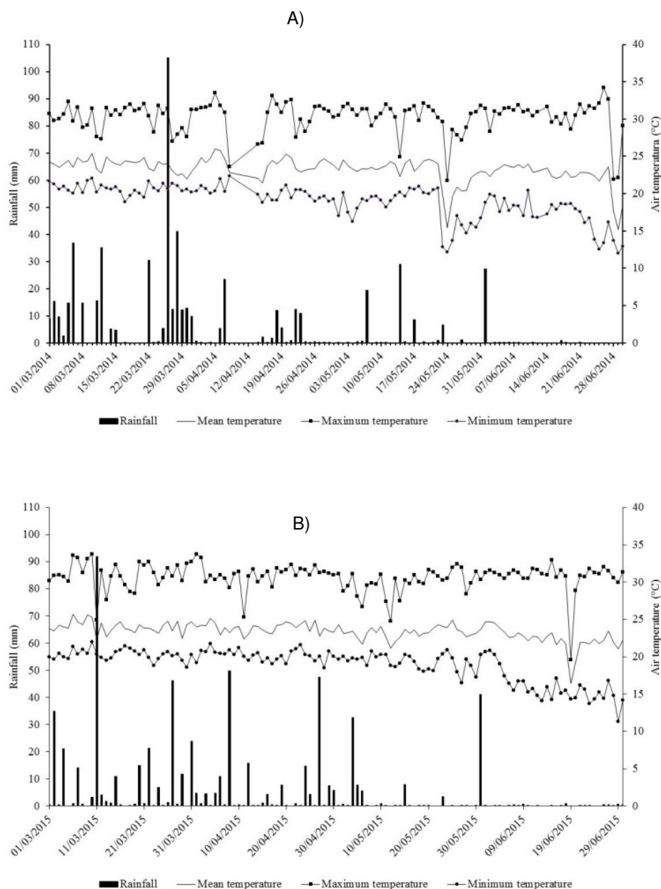
Fig. 2. Rainfall and thermal averages in the experimental area between March and June of 2014
