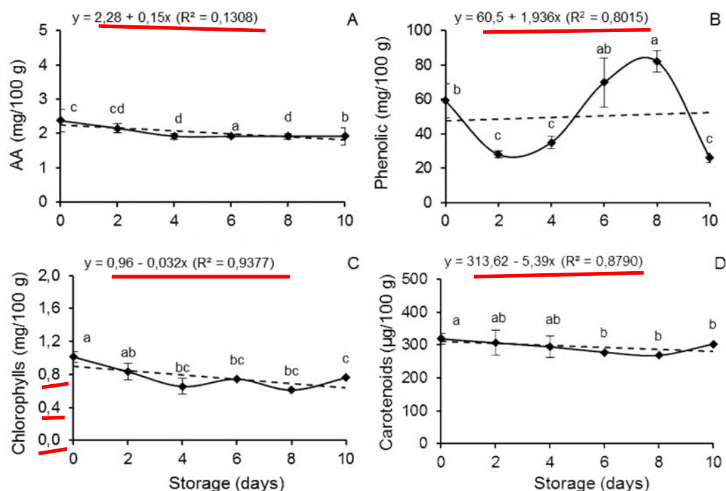
Fig. 3. Ascorbic acid (A), phenolic compounds (B), chlorophylls (A) and carotenoids (B) in minimally processed young cladodes of the 'Mexican elephant ear' palm.
