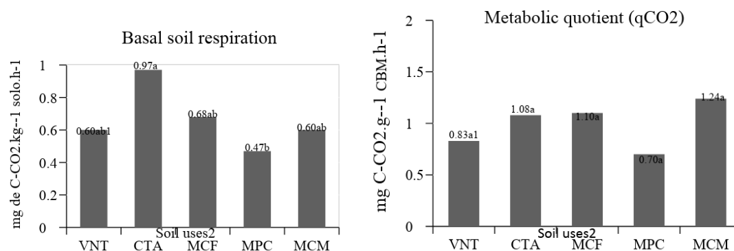
Figure 2. Behavior of the different parameters of biological activity in soil samples from areas under different uses. 1 Averages followed by the same letter do not differ among themselves by the Tukey test at 5% probability. 2 VNT = native vegetation of caatinga; CTA = pasture of tanzania grass intercropped with algarobeira; MCF = corn intercropped with beans in conventional cultivation; MPC = corn in monoculture under conventional cultivation and MCM = corn in monoculture under minimum cultivation.
