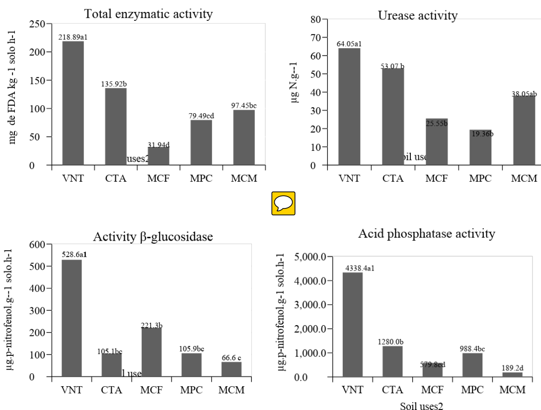
Figure 1. Behavior of the different enzymatic parameters in soil samples from areas under different uses. 1 Averages followed by the same letter do not differ among themselves by the Tukey test at 5% probability. 2 VNT = native vegetation of caatinga; CTA = pasture of tanzania grass intercropped with algarobeira; MCF = corn intercropped with beans in conventional cultivation; MPC = corn in monoculture under conventional cultivation and MCM = corn in monoculture under minimum cultivation.
