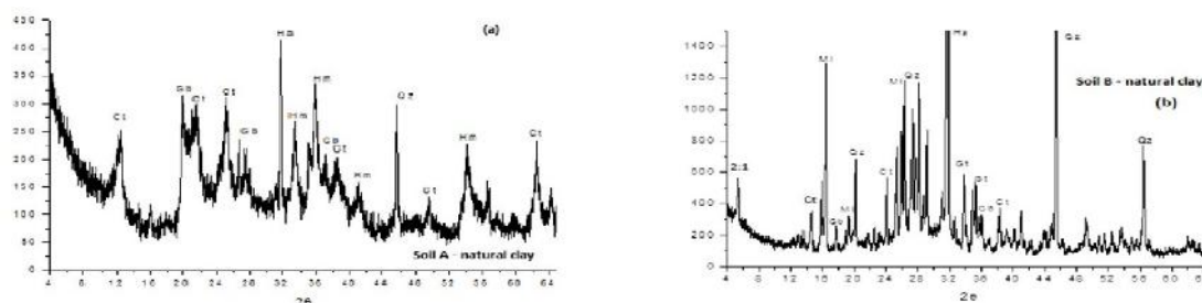
Fig. 1. X-ray diffraction (CuK \alpha radiation) of clay fraction of soil A (a) and soil B (b). Ct - caulinite, 2:1 - secondary mineral 2:1, Hm - hematite, Qz - quartz, Gb - gibbsite, Ha - halite, Mi - mica, Gt - goethite
