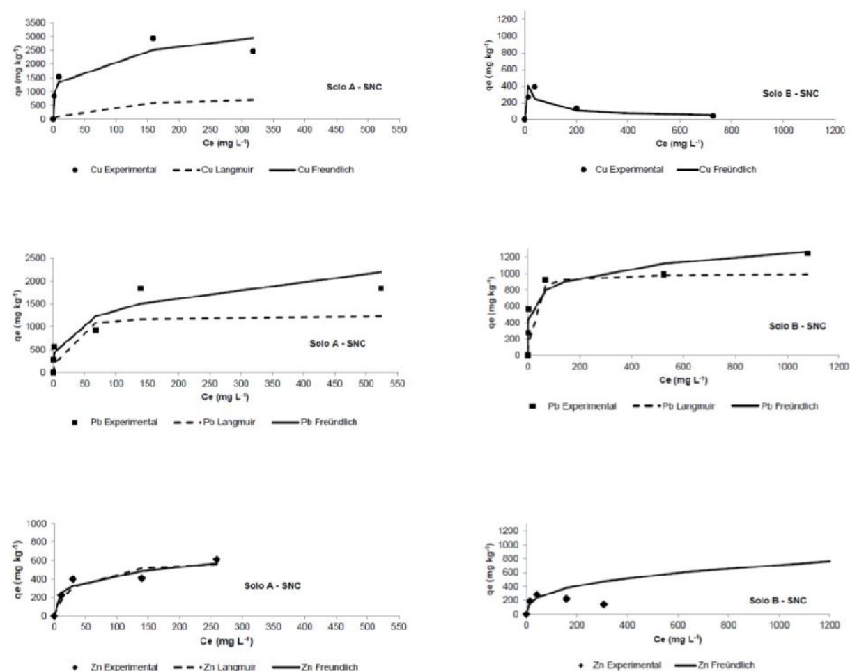
Fig. 2. Cu, Pb and Zn adsorption isotherms in a non-competitive system for clay soil (Soil A) and sandy soil (Soil B).
