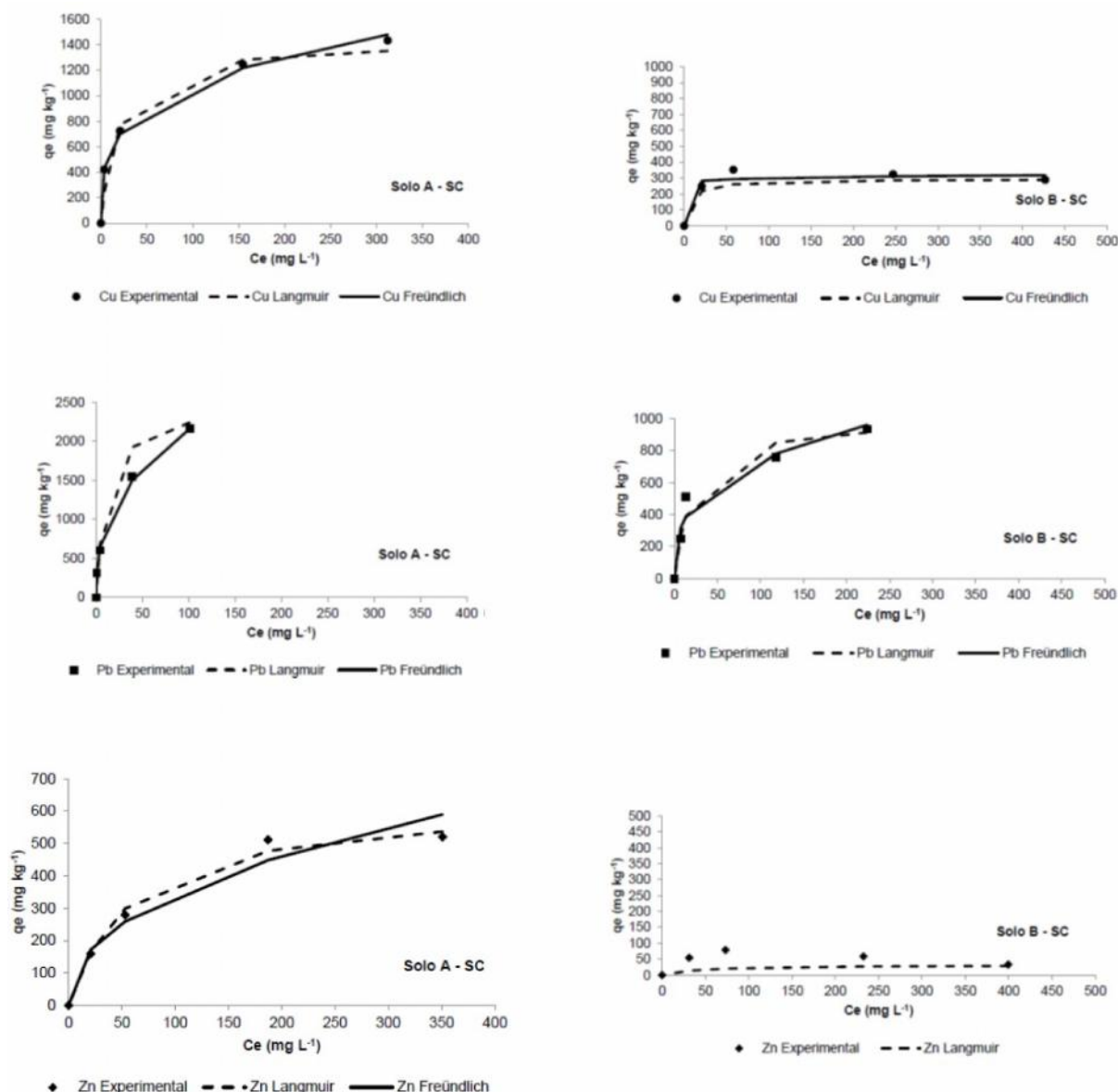
Fig. 3. Cu, Pb and Zn adsorption isotherms in a competitive system for clay soil (Soil A) and sandy soil (Soil B).
