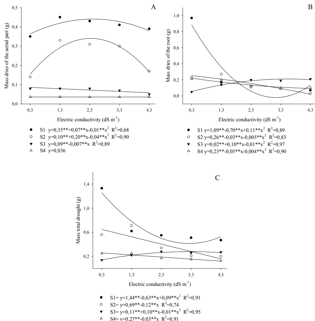
Figure 3. Mass dries of the aerial part (A); root (B) and total (C) of melon plant plantules (Amarelo Ouro) in function of different substrates and saline levels, UFCG, Pombal, 2018.
