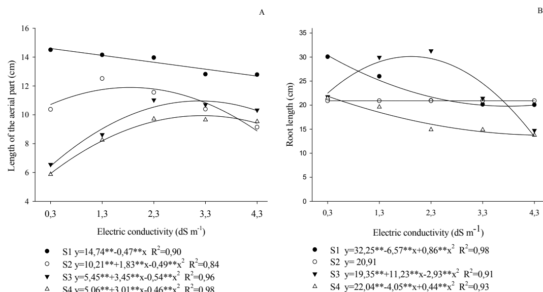
Figure 1. Length of the aerial part (A) and root (B) of melon plant plantules (Amarelo Ouro) in function of different substrates and saline levels, UFCG, Pombal, 2018.
