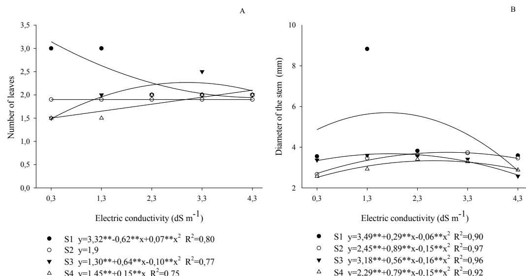
Figure 2. Number of leaves (A) and diameter of the stem (B) of melon plant plantules (Amarelo Ouro) in function of different substrates and saline levels, UFCG, Pombal, 2018.
