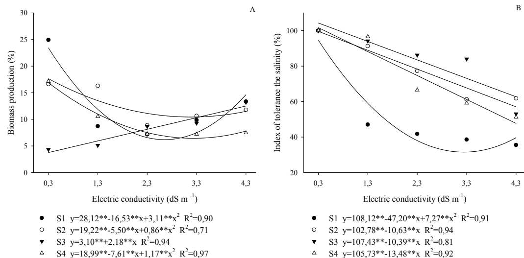
Figure 4. Biomass production (A) and index of tolerance the salinity (B) of melon plant plantules (Amarelo Ouro) in function of different substrates and saline levels, UFCG, Pombal, 2018.
