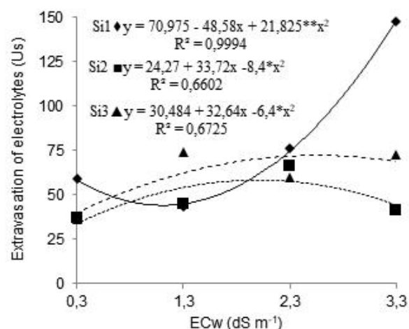
Figure 4. Extravasation of electrolytes in Cucumis melo L., as a function of different salinities
