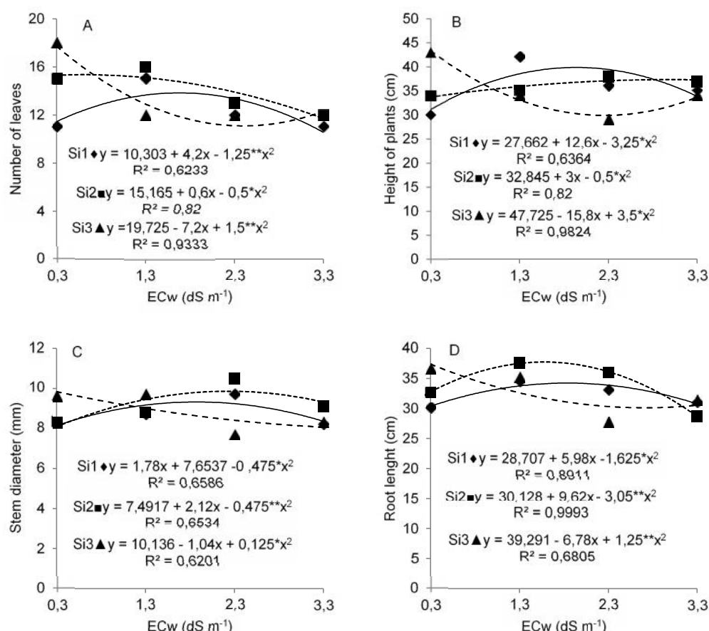
Figure 1. Number of leaves (A), height of plants (B), stem diameter (C) and root length (D), of Cucumis melo L., as a function of different salinities of irrigation water and silicon doses.
