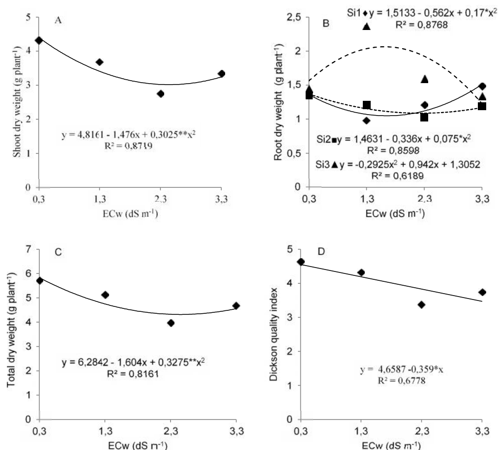
174 Figure 3. Shoot dry weight (A), root dry weight (B), total dry weight (C) and Dickson quality 175 index (D) of Cucumis melo L., as a function of different salinities of irrigation water and silicon 176 doses. 177 ** P < 0.01 ; * P < 0.05
