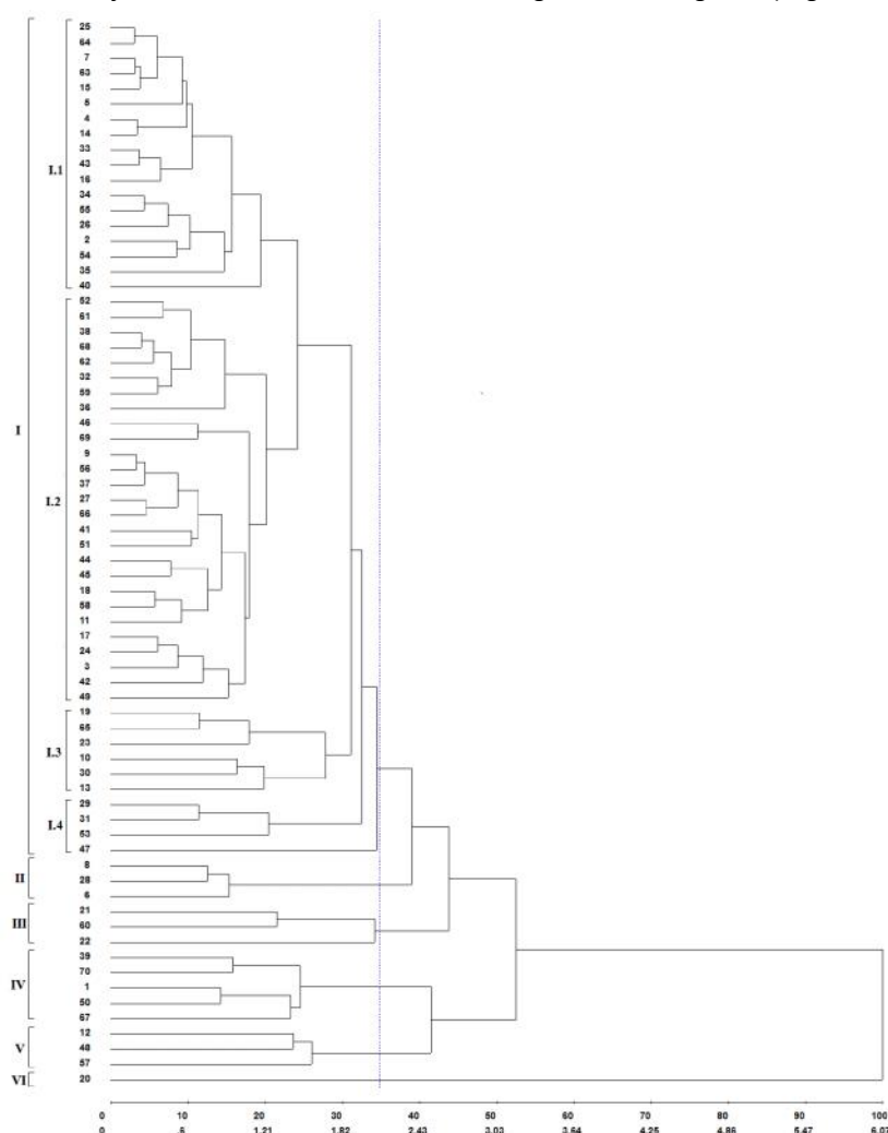
Figure 2. UPGMA dendrogram obtained from the dissimilarity matrix ( D^2 ) of the 70 C. procer a accessions based on 23 agronomic characters. The cophenetic correlation coefficient was 0.777. The dotted line represents the cutoff point based on the methodology proposed by MOJENA (1977).
