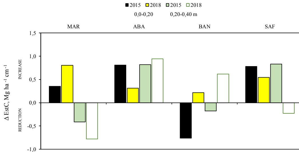
170 171 Figure 4. Variation of organic carbon stocks ( \Delta\text{EstC} ) at depths of 0.0-0.20 and 0.20-0.40 m in relation to the 172 native forest system (MN) in areas of organic management in the semi-arid Bahia under different uses: (SAF) 173 agroforestry system, (MAR) passion fruit cultivation in monoculture, (ABA) pineapple cultivation in 174 monoculture, (BAN) banana cultivation in consortium. Positive values indicate an increase in the organic carbon 175 stock in relation to the MN system.
