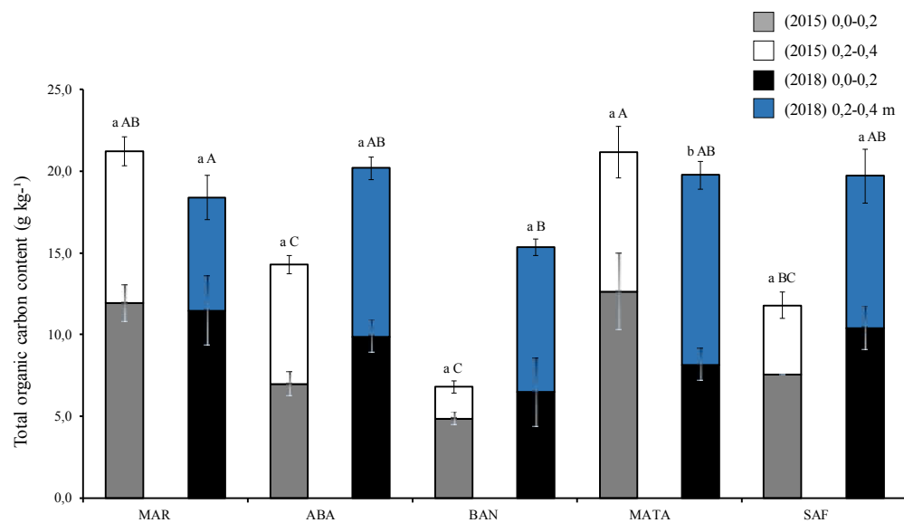
Figure 3. Mean values of total organic carbon at depths of 0.0-0.20 and 0.20-0.40 m in areas under organic production system in the Bahian semi-arid under different uses: (SAF) agroforestry system, (MAR) cultivation of passion fruit in monoculture, (ABA) cultivation of pineapple in monoculture, (BAN) banana cultivation in a consortium and native forest system (MN). * Vertical lines represent the standard deviation and averages followed by equal lowercase letters do not differ the levels for years of handling within each system and capital letters do not differ between systems within each crop year. * Chart statistic referring to depth of 0.0-0.20 m.
