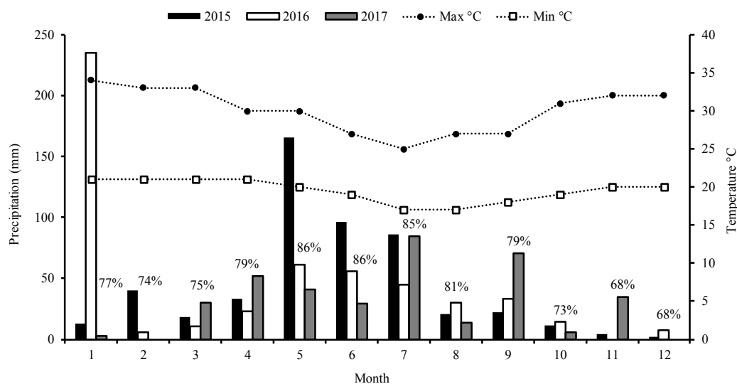
Figure 1. Mean monthly values of temperature (°C), precipitation (mm) and humidity (%) during the three consecutive years of the evaluation interval of the experimental area (2015 to 2017). Feira de Santana, Bahia.
